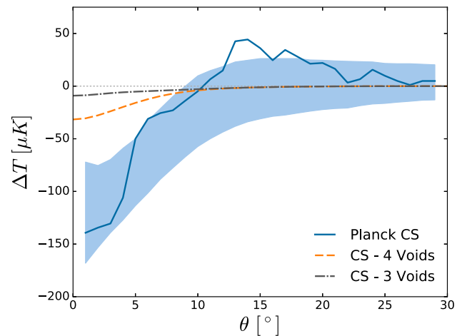
Figure 8. The Cold Spot temperature profile (Planck Collaboration et al. XVI 2016b, blue line) and the ISW imprints of the 3- and 4-void models (grey dot-dashed and yellow dashed, respectively) fitted to the Cold Spot region. The void temperature profiles from Table 3 have been summed and the result fitted to equation 3 of Naidoo et al. (2016). The shaded region (light blue) is the 68 per cent confidence interval from the coldest spots identified in Gaussian simulations (see fig. 6 of Nadathur et al. 2014).
