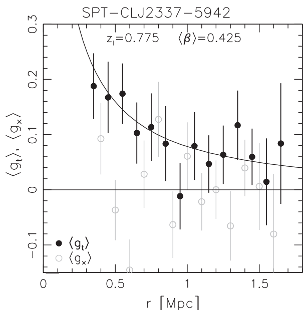
Figure 16. Tangential reduced shear profile (black solid circles) of SPT-CLJ2337–5942 centred on the X-ray centroid and obtained by combining the profiles of all contributing magnitude bins of the ACS-only plus the ACS+FORs2 selection (see Section 7.2). The curve shows the correspondingly combined best-fitting NFW model prediction obtained by fitting the data in the range 500 \text{ kpc} \leq r \leq 1.5 \text{ Mpc} and using the Diemer & Kravtsov (2015) concentration–mass relation. The grey open circles indicate the 45 degrees-rotated reduced cross-shear component, which is a test for systematics, shifted by dr = -0.05 \text{ Mpc} for clarity. The corresponding plots of the other clusters are shown in Appendix G.
