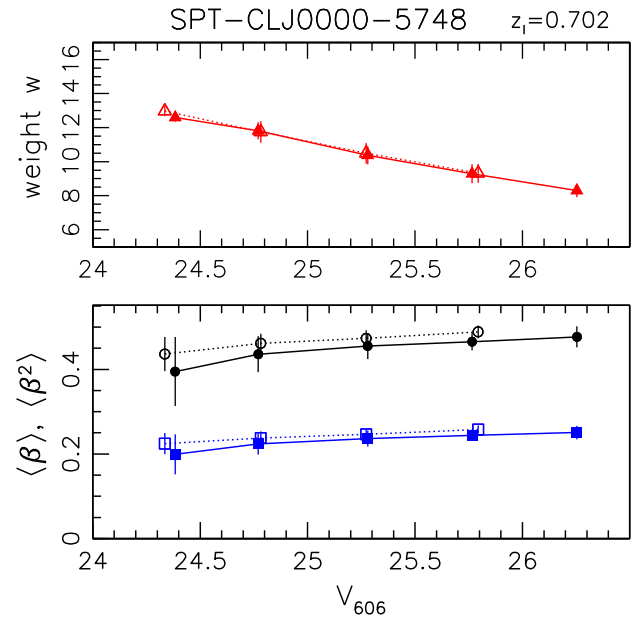
Figure 8. Analysis of SPT-CL J0000–5748 as a function of V_{606} magnitude, where the solid (open) symbols correspond to the ACS-only (ACS+FORS2) analysis. Top: Mean weak lensing shape weight w with error-bars indicating the dispersion from all selected galaxies in the magnitude bin. Bottom: \langle \beta \rangle (circles) and \langle \beta^2 \rangle (squares) with error-bars showing the dispersion of their estimates computed from all CANDELS sub-patches (see Section 6.6), thus indicating the expected line-of-sight variations for the field sizes of our cluster observations.
