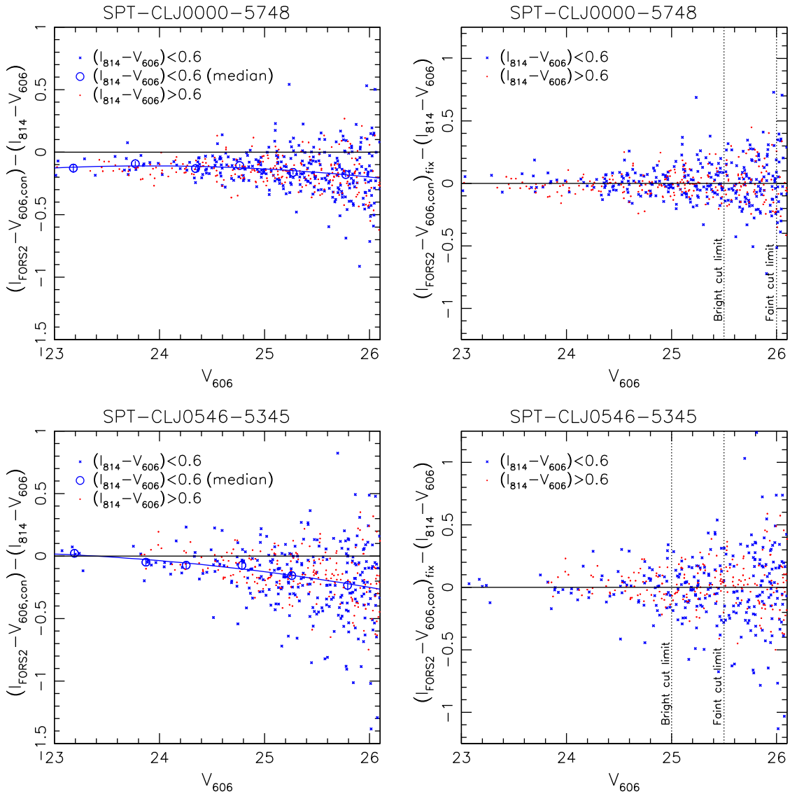
Figure D1. Details on the colour selection for SPT-CLJ0000-5748 (top) and SPT-CLJ0546-5345 (bottom). Left: Difference between the colour (I_{\text{FORS2}} - V_{606,\text{con}}) measured with the FORS2 I band and the convolved HST/ACS F606W images, and the colour (I_{814} - V_{606}) measured from the unconvolved HST/ACS data in the inner cluster region, as a function of V_{606} . Small blue crosses indicate blue galaxies with (I_{814} - V_{606}) < 0.6 , while red points show red galaxies with (I_{814} - V_{606}) > 0.6 . The open circles mark the median values for the blue galaxies within 0.5 mag wide magnitude bins, with error-bars indicating the uncertainty on the mean for a Gaussian distribution, and the curve showing their best-fitting second-order polynomial interpolation. The right-hand panels show the same data after subtraction of this function. We sample the photometric scatter distribution for the ACS-FORS2 selection from this distribution of offsets. Because of the lower scatter in the deeper FORS2 data of SPT-CLJ0000-5748 we can include fainter galaxies in the ACS-FORS2 selection than for SPT-CLJ0546-5345 (see Table 2 and the indicated bright/faint cut limits).
