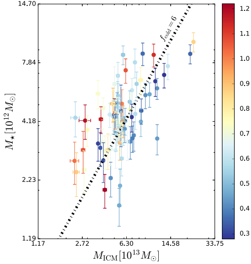
Figure 10. The relation between the stellar mass M_* and the ICM mass M_{\text{ICM}} among the 84 clusters. This relation is approximated as M_* = 4 \times 10^{12} M_{\odot} \times \left( \frac{M_{\text{ICM}}}{5.7 \times 10^{13} M_{\odot}} \right)^{0.60} by assuming no redshift trends for M_* -to- M_{500} and M_{\text{ICM}} -to- M_{500} relations. Each cluster is colour-coded by the redshift, while the confidence levels (grey area) of the M_* -to- M_{\text{ICM}} relation are fully marginalized and extracted from the MCMC chains of the M_* -to- M_{500} and M_{\text{ICM}} -to- M_{500} relations. The dashed line indicates the cold baryon fraction of 6 per cent at the pivot mass and redshift.
