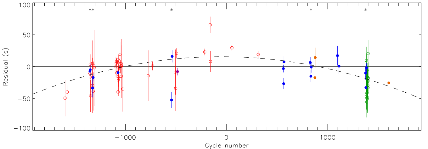
Figure 2. Plot of the residuals of the timings of mid-transit versus a linear ephemeris. The results from this work are shown with filled circles: blue for the Danish telescope, orange for the SAAO 1.0 m, and purple for the NTT. Published results are shown using open circles: red for the literature data collected by B19 and green for the TESS timings from B19. The dotted line shows the difference between the best-fitting linear and quadratic ephemerides. Grey asterisks have been placed near the top of the figure to indicate transit times measured from a light curve with a spot crossing event.
