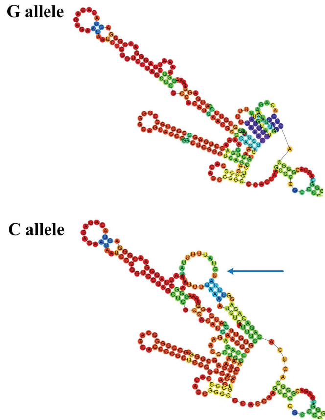
Figure 2. In silico analyses predicting secondary structure of HOTAIR with RNAfold. The arrow indicates alteration in structures caused by rs7958904 G/C variant.
