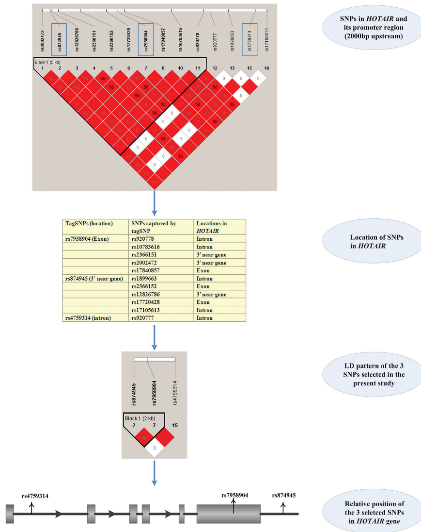
Figure 1. Overall flow of SNP selection and relative location of the three selected tagSNPs in HOTAIR. TagSNPs selected in Haploview were marked with blue line box
