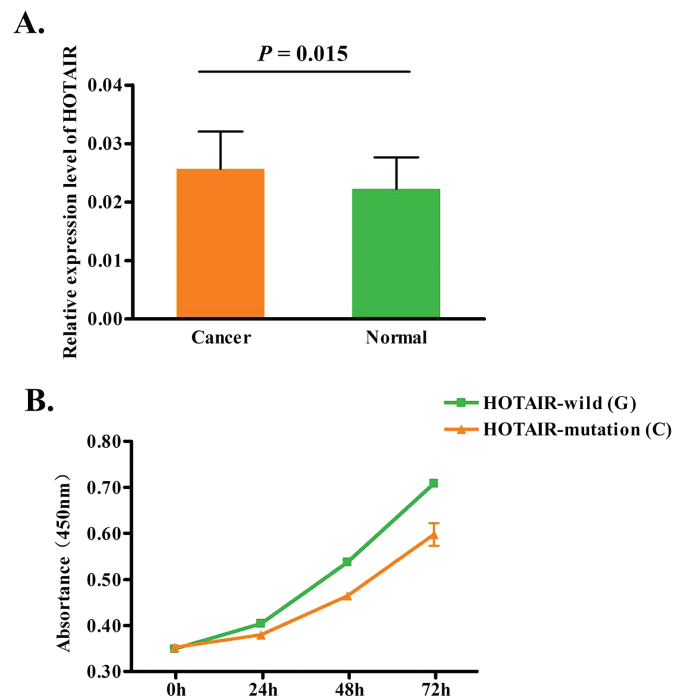
Figure 3. (A) Expression level of HOTAIR in colorectal cancer tissues was significantly elevated than in adjacent normal tissues. (B) Effects of HOTAIR -G or HOTAIR -C overexpression on colorectal cancer cell proliferation, detected by CCK-8 assay. Proliferation of cells transfected with HOTAIR -C plasmid was significantly decreased compared with those transfected with HOTAIR -G plasmid. Detailed data are shown in Supplementary Table 4 , available at Mutagenesis Online .
