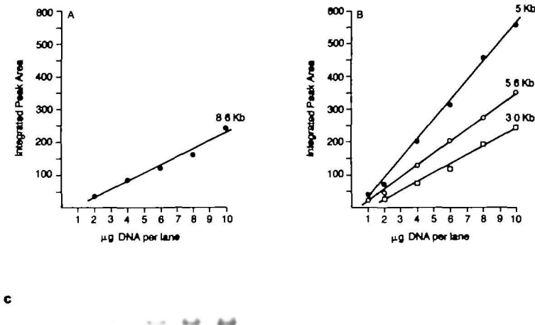
Figure 4. Proportionality of probe detection signals. Various amounts of Hind III digested human genomic DNA were electrophoresed on a 0.7% agarose gel, subjected to Southern transfer, and blot and hybridization with the PGK-5 cDNA probe. Lanes were scanned with a 525 nm laser source with a beam-width 30% larger than the width of the lanes being scanned. Integrated peak areas were plotted vs. the amount of total genomic DNA loaded. Plots of each fragment shown were taken from a single film. An exception is the 8.6 kb fragment which was analyzed on a separate exposure because of grain saturation in the original exposure. (A) Peak area under the 8.6 kb fragment vs. amount of total genomic DNA loaded. (B) Area vs. amount loaded for the 3.0, 5.0 and 5.6 kb fragments. (C) Portion of autoradiogram showing the 5.0 kb fragment with increasing (left to right) amounts of total genomic DNA loaded.
