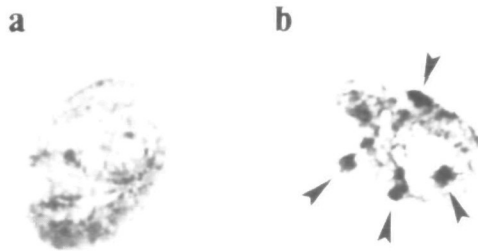
Figure 6. Barr body analysis performed on isolated nuclei. Nuclei were prepared by the same procedure used throughout this report, and subjected to the Barr body analysis described in "Materials and Methods."
