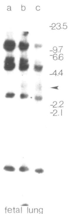
Figure 8. Nuclei from human fetal lung tissue were treated with increasing levels of DNase I as in previous figures. The DNA was purified, restricted with Hind III and blot hybridized to the PGK probe. The arrow indicates the position of the 3.9 kb DNase I-induced sub-band. a, 2 µg/ml DNase I; b, 5 µg/ml; c, 10 µg/ml.
