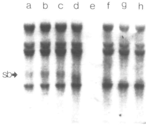
Figure 2. Terminal digestion of the DNase I sensitive site by Bal31 . DNA was purified from nuclei digested with DNase I to a level which maximizes sub-band material. The purified DNA was digested for increasing (left to right) times with the exonuclease, Bal31 . The Bal31 reactions were stopped by adding EGTA. The DNA was then restricted with HindIII , subjected to Southern blotting and hybridization to the probe to PGK encoding sequences. a) No Bal31 ; b) 30 min Bal31 digestion; c) 60 min; d) 90 min; e) Molecular weight markers - not visible; f) 2 hr; g) 3 hr; h) 4 hr. "Sb" marks the position of the sub-band which is selectively attacked by Bal31 .
