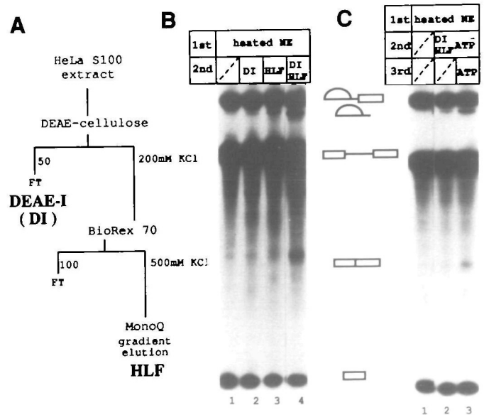
Figure 3. Requirement of HLF and DEAE-I for the formation of spliceosome IIb. (A) Scheme for the purification procedure of DEAE-I and HLF from the HeLa S100 fraction. The KCl concentrations of loading buffers or elution buffers are indicated. FT represents flow-through fractions. (B) The immobilized pre-mRNA was first incubated with the heated nuclear extract for 90 min. The second incubation was in 20 µl reaction mixtures containing 12 µl DEAE-I (lane 2), 12 µl HLF (lane 3), or 6 µl DEAE-I and 6 µl HLF (lane 4). After incubations, RNAs were analyzed as in Figure 1. (C) The second incubation was with equal volume of DEAE-I and HLF in the absence of ATP and creatine phosphate for 30 min. The third incubation was in buffer E containing 1 mM ATP for 1 hr. RNAs were analyzed as in Figure 1.
