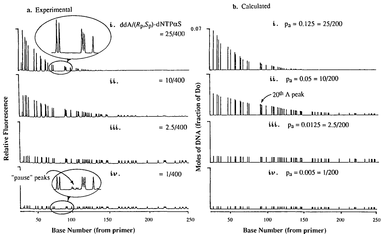
Fig. 10. Comparison of experimental (panel a) and calculated (panel b) termination patterns with variable ratios of ddATP/dNTP \alpha S. The experimental extension reactions contained M13mp18, FAM-labeled -21 primer, Mn^{2+} , Mg^{2+} , T7 DNA polymerase, pyrophosphatase and ratios of ddATP/( R_p, S_p )-dNTP \alpha S varying from 25 \mu M/400 \mu M to 1 \mu M/400 \mu M. (The ratios of ddATP to the active isomers of the dNTP \alpha S's were from 25 \mu M/200 \mu M to 1 \mu M/200 \mu M.) The fluorescence patterns were collected through the 580 nm filter; all the peaks are shown on the same scale. The first peak in each panel is the 5 th A peak following the primer. The calculated termination patterns were obtained by entering the M13mp18 sequence, varying the termination probabilities of A-termination from 0.125 to 0.005 and setting the probabilities of terminating in C, G and T to zero. The linear regression analysis of each fluorescent peak vs. its corresponding calculated molar quantity gave correlation coefficients for panels i. - iv. of 0.995, 0.989, 0.969, and 0.969.
