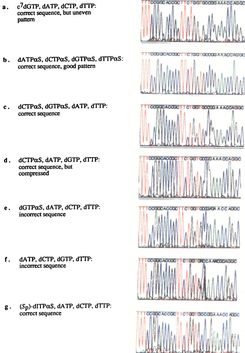
Fig. 7. Effects of different dNTP compositions on the resolution of a hairpin sequence. The sequence consisted of an 11 base pair stem and six base loop (5'-TTTCCGGCACCGCTTCTGGTGGCGGAAA-3'). Each extension reaction contained M13mp18 annealed to a 17-bp primer at base 6571, four fluorescein-labeled terminators, Mn 2+ , Mg 2+ , T7 DNA polymerase and pyrophosphatase.
