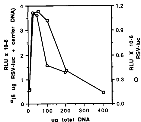
Figure 2. Maximum luc activity attained with reporter plasmid alone or with bluescript carrier DNA. RSV-luc was transfected alone at amounts between 5 and 200 \mu\text{g} (circles). Five \mu\text{g} RSV-luc was transfected with increasing amounts of bluescript carrier, up to 400 \mu\text{g} (squares).
