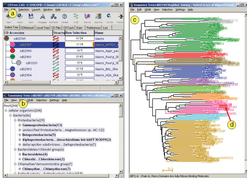
Figure 2. CDTree default display, as launched from a web browser, showing a curated domain hierarchy with an embedded user query sequence. A protein sequence found in NCBI's Entrez database was inspected for the presence of conserved domains. The user has followed links from one of the domain footprints annotated on the model, and inspected a particular domain model, cd02907. From the CD summary page, as shown in Figure 1, CDTree was launched as a helper application. The main window (a) presents the organization of the conserved domain hierarchy, as already visible on the CD summary page (Figure 1). In this case, cd02749 or 'Macro' is a generic 'parent' model, which has been split up into several more specific 'children'. The sequence tree shown in panel (c) provides evidence for this particular subfamily structure. Groups of branches rendered in the same color correspond to alignment tracks that have been assigned to a particular subgroup. Sequence trees are always calculated from the curated CD alignments; in this particular example, the distance data have been obtained from pair-wise alignment scores. Aligned residue pairs are scored with the BLOSUM62 matrix. Pair-wise scores are subtracted from the highest observed pair-wise score to yield distances, and the distance units plotted here correspond to BLOSUM62 scores. By default, a taxonomy viewer window is opened as well (b). Users may select and highlight whole branches in the sequence tree view and examine corresponding highlights in the taxonomy viewer, to understand the taxonomic scope of particular subfamilies, or select/highlight taxa in the taxonomy viewer and examine their distribution in the sequence tree. In this example, a user query sequence has been added to one of the models, cd02907. cd02907 gave the best scoring hit in a database search for a particular region of the user's query sequence. In the sequence tree display, the user query is highlighted by default (d). It appears that the user query is a typical member of this particular subfamily, as it clusters tightly with all the other members, and therefore transfer of annotation from the model to the sequence - or functional inference - may be appropriate.
