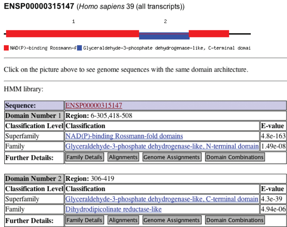
Figure 2. Domain architecture and assignment details for the Ensembl protein ENSP00000315147 from human. Shown are the superfamily and family classification and associated E -values for two domains. Links to further family details, alignments between the SUPERFAMILY model and the protein, assignments for the human genome and domain combinations in which the superfamily domain occur in are included for each domain.
