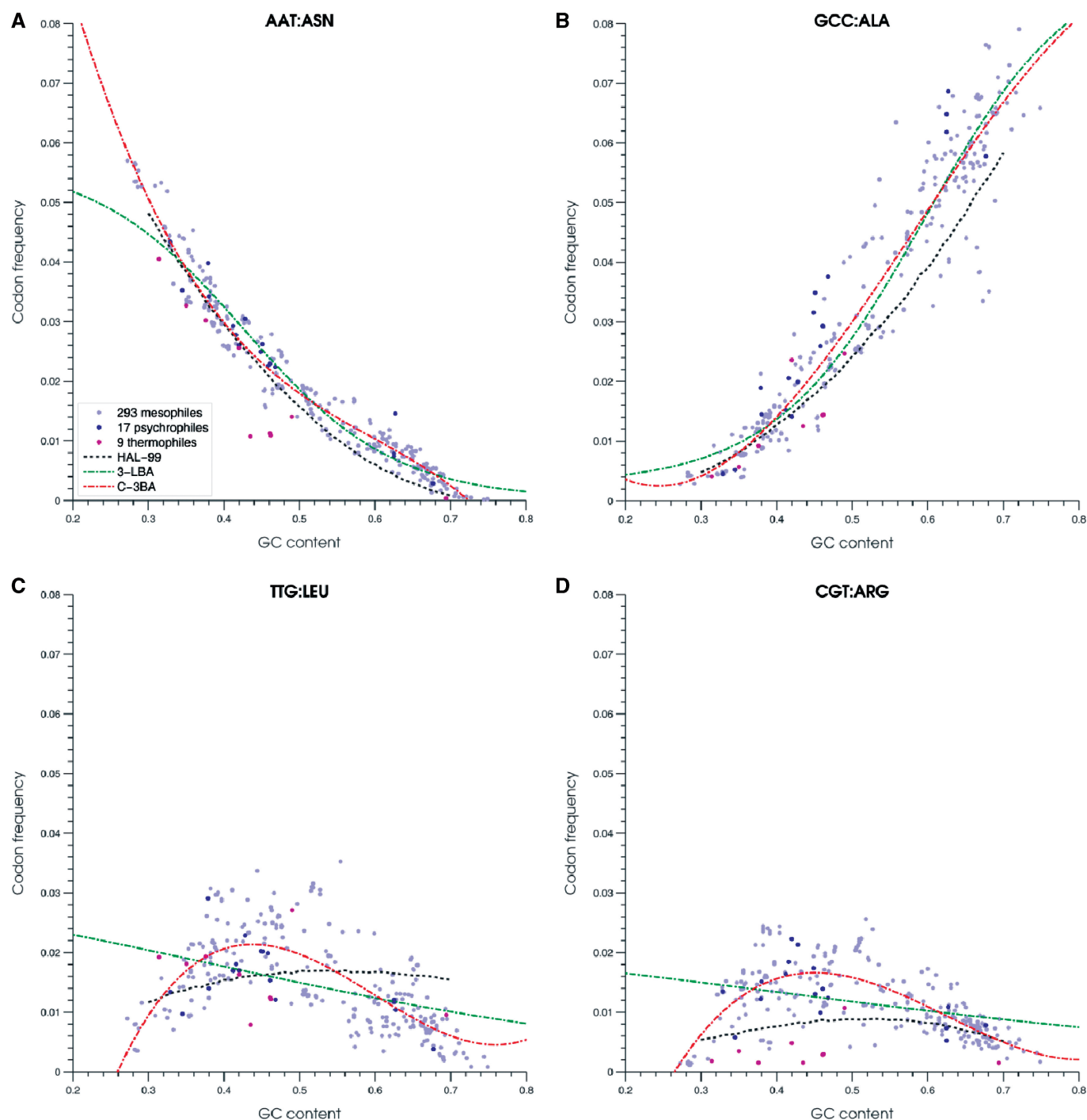
Figure 3. Characteristic cases of codon frequency dependence on genome GC content. Each panel shows observed frequencies of a given codon in 319 bacterial genomes. Mesophilic, psychrophilic and thermophilic species are shown as light blue, dark blue and purple dots, respectively. Three techniques of approximating dependence of codon frequency from genome GC content are illustrated: 1999 heuristic model (HAL-99, black dotted line); logistic regression (3-L, green dotted line); and order three polynomial regression (C-3, red dotted line). Plots for 61 codons are available at http://exon.gatech.edu/GeneMark/metagenome/Training/PlotPDF/BAC2D.pdf .
