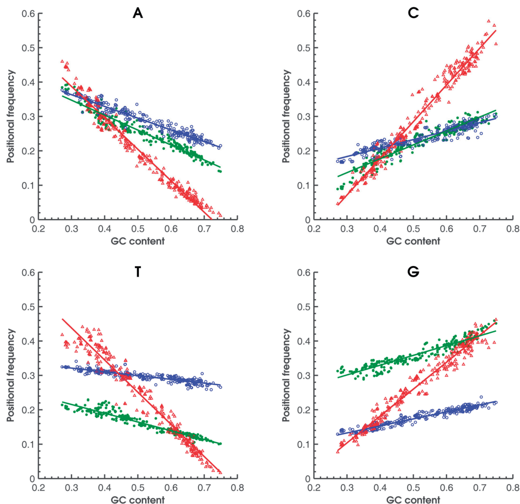
Figure 1. Observed frequencies of 4nt in the three codon positions (first: green; second: blue; third: red) as functions of genome GC content for 319 bacterial genomes. Nucleotides G and T have more contrast in frequencies in the first and second position in comparison with A and C. Frequencies in the third codon position are most sensitive to genome GC content.
