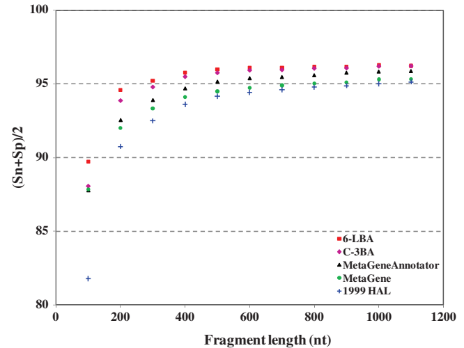
Figure 8. Gene prediction accuracy of GeneMark.hmm with three different heuristic models, as well as MetaGene and MetaGeneAnnotator observed on the sets of sequence fragments with length from 100 to 1100 nt from 50 microbial chromosomes.
