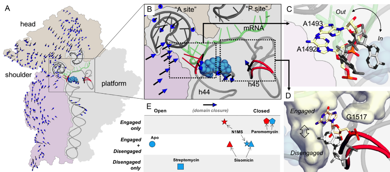
Figure 3. Sisomicin and NIMS binding to the 30S decoding complex induces an intermediate state of 30S domain closure. (A) The 30S ribosomal subunit illustrating the location of the drug binding pocket and the site of the h44–45 interactions. The drug is shown with blue spheres. The 30S subunit contour is shown with three different colored regions of interest, and the portion of the rRNA making helices h44 and h45, and the ASL Phc and mRNA moieties are shown as gray ribbons. The first principal component (see the text) is displayed as a vector field from the ensemble average structure. Note that smaller displacements were filtered out, and the arrows displayed are arbitrarily scaled, for clarity. More local motions of interest are further highlighted in red in the decoding center. (B) Detailed view of the decoding center displaying the drug binding pocket, where A1492 and A1493 (red sticks in left box) are displaced in response to aminoglycoside binding. The two h45 states, engaged and disengaged are also shown on the right (red ribbon in right box). (C) Detailed view of the flipping bases, in the context of the decoding center where the A-site tRNA (top left, gray), the mRNA (green) can be seen close to the outward flipped bases, and the aminoglycoside molecule (blue sphere) is seen superposed with the inward flipped state of the same bases. (D) Engaged and disengaged conformations of h45. The pocket in which G1517 is engaged, made in part by h44, is shown as a surface. Proximity to the drug (spheres in the background) binding site is apparent. (E) Ordering of the apo-30S (circle) structure and the streptomycin (square), sisomicin (triangle), NIMS (star) and paromomycin (pentagon) 30S decoding complex structures. Blue represents cryogenic structures, red represents ambient temperature structures studied along the first principal component extracted from their conformational ensemble. The vertical scale shows h45 disengagement, engagement or equilibrium in the corresponding crystal structure.
