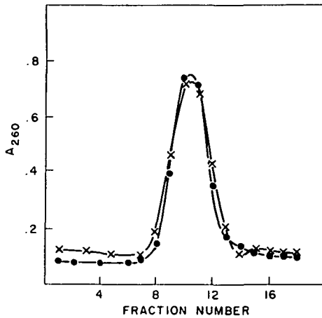
Figure 1 Sucrose gradient sedimentation of reconstituted 30S particles. (—•—) using unoxidized 16S rRNA. (—x—) using periodate oxidized, PSC-conjugated 16S rRNA.
