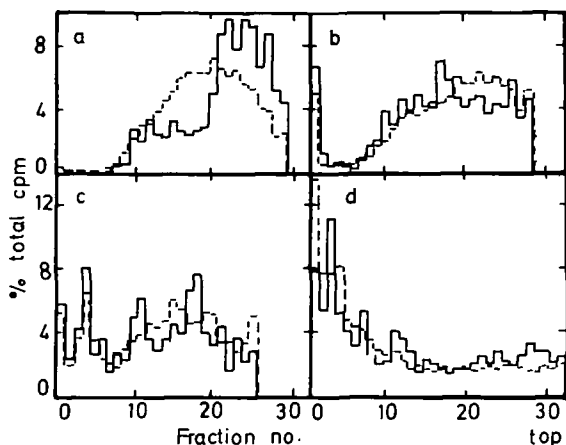
Fig. 3. Rejoining of double strand breaks in 1BR (—) or AT3BI (---) after treatment for 1 h with 500 \mu\text{g}/\text{ml} bleomycin and incubation for 0 (a), 0.5 (b), 1 h (c), 2 h (d). Centrifugation at 7,000 rpm for 16 h on neutral sucrose gradients.
