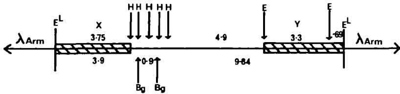
Figure 3. Restriction endonuclease map of \lambda CH-01 insert DNA. Map distances are shown in kilobase pairs. Restriction sites are shown as B_g = BglII, E = EcoRI, H = HindIII. E^L denotes the boundaries of the insert (the library was constructed with EcoRI linkers; see Materials and Methods). The blocked-in regions represent fragments containing histone coding regions (Fig. 1 and unpublished results). The exact number and location of HindIII sites situated between fragment X and the 4.9 kb non-coding fragment are not known. Because the several HindIII fragments referred to are small, it is not yet known whether they contain any coding regions.
