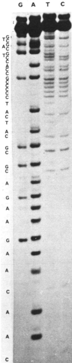
Figure 5. Autoradiogram of DNA sequencing gel from HaeIII fragment 9 (see Fig. 4). Single-stranded 5'-labelled fragments were sequenced by the method of Maxam and Gilbert (20) and bands resolved on 20% polyacrylamide gels (0.5 mm thick). The DNA sequence shown corresponds to a portion of the chicken H2A gene (Fig. 6).
