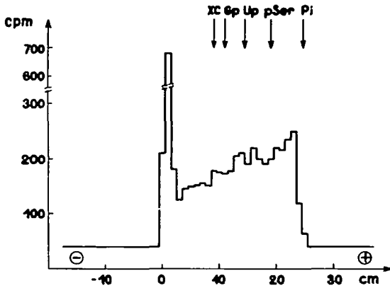
Fig. 5. Paper electrophoresis of VPgA-pUp hydrolyzed with 4 M HCl for 6 h at 105°C.
