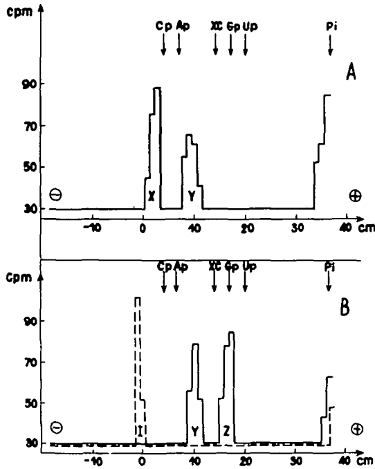
Fig. 3. Paper electrophoresis at pH 3.5 of nucleotide-peptides treated with bacterial alkaline phosphatase and pronase. A, nucleotide-peptide II. B, nucleotide-peptide I (---) and nucleotide-peptide III (—). 700 cpm and 640 cpm of treated nucleotide-peptide II and III, respectively, were applied.
