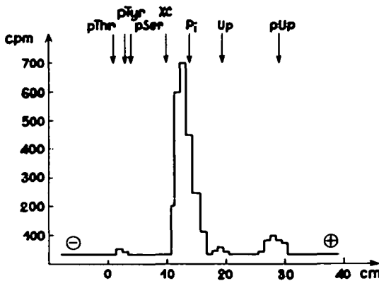
Fig. 6. Paper electrophoresis at pH 1.7 of fractions II-24 (Fig. 5).
