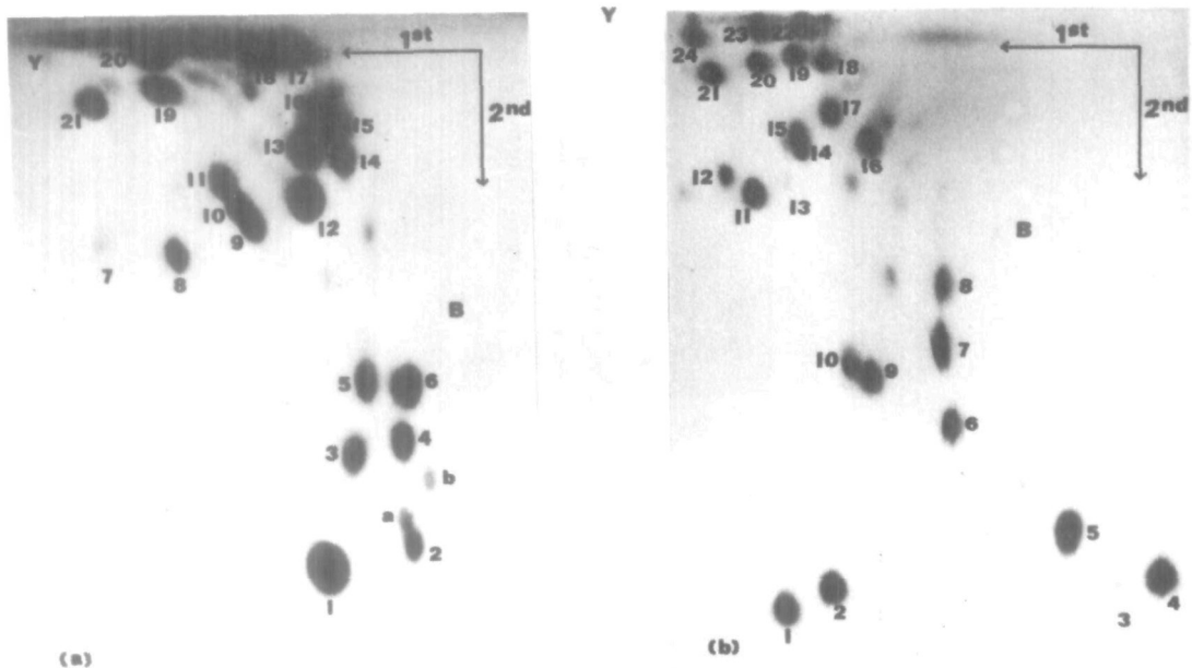
Figure 3: Two-dimensional fingerprints of a) T1 RNase-digested and b) RNase A-digested ^{32}\text{P} -labelled sea urchin embryo 5S rRNA. Oligonucleotide numbers correspond to the data presented in Tables I and II. ^{32}\text{P} -labelled 5S rRNA was purified as described in the Materials and Methods. Electrophoresis was on cellulose acetate (Cellogel) in 7 M urea/pyridinium acetate, pH 3.5, for the first dimension and in 7% formic acid on DEAE paper for the second. B and Y mark the positions of the blue (xylene cyanole FF) and yellow (orange G) dye markers. Arrows indicate the directions of the first and second dimensions; the origin, however, is not included in the sections of the autoradiograms photographed. As part of the search for oligonucleotides derived from the 5' and 3' termini of 5S rRNA, all minor oligonucleotides visible in the fingerprints, but not numbered, were analyzed. With the exception of T2, T7, and P13, which are discussed in the text, these minor oligonucleotides did not have the properties appropriate for 5' and 3' ends.
