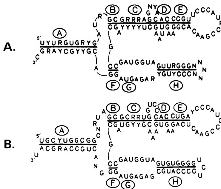
Figure 4: "Wishbone" Models for Prokaryotic 5S rRNA. General models of 5S rRNA from gram positive bacteria and from gram negative bacteria are shown in (A) and (B) respectively. Constant specific nucleotides are indicated by A, C, G, U, with constant purines indicated by R and pyrimidines by Y. Non-conserved bases are labelled N. The data were compiled from Hori and Osawa (45). Constant, here, means present in at least 12 of 15 of gram-negative bacteria (lines 25-PHO to 39-ECKD) or in at least 11 of 14 gram-positive bacteria (lines 41-BME1 to 54-CPA). A. nidulans , P. fluorescens and T. aquaticus were not counted. Since their list contains many variants of E. coli and Bacillus , it is probably not representative sampling of prokaryotes.
