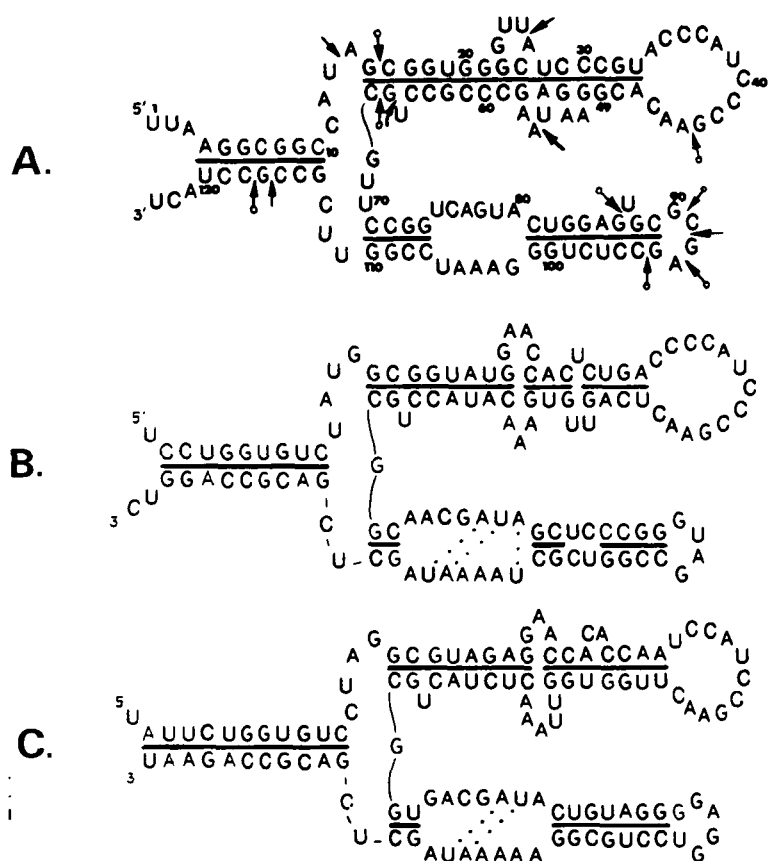
Figure 7: 5S rRNA from a Halophilic Bacteria, a Blue-Green Bacteria and a Chloroplast. (A) The best filtered solution (3 of 4) for H. cutiribrium . (B) The best filtered (12 of 14) solution for A. nidulans 5S rRNA and for (C) L. minor chloroplast (3 of 4). No chemical modification or enzymatic cleavage data are available for A. nidulans and L. minor . This lowest energy Lemna minor structure corresponds to a slightly different alignment in the vicinity of helix D than in Figure 3.
