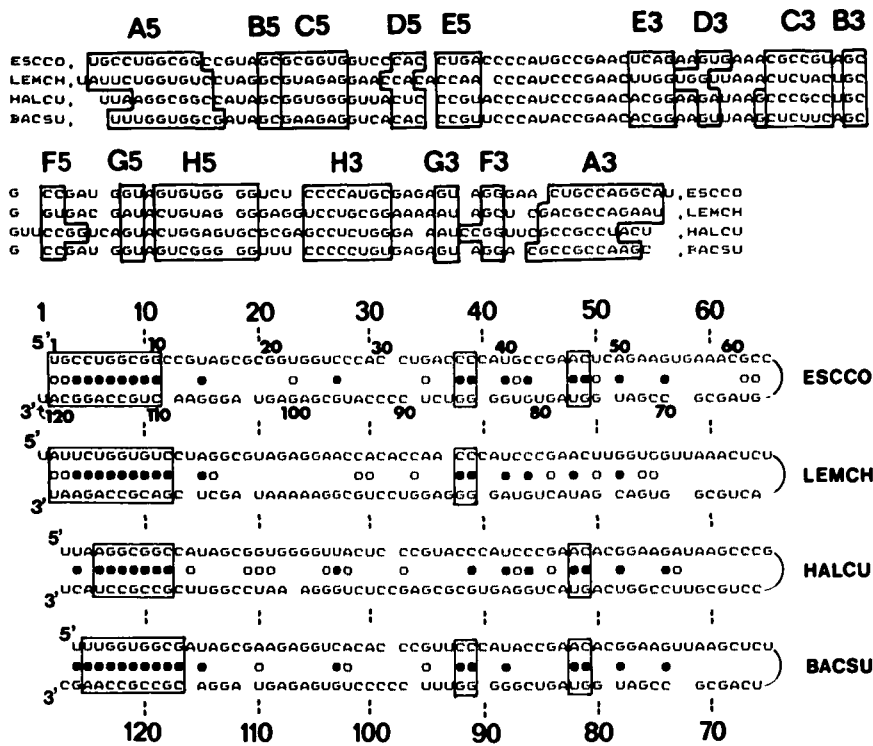
Figure 3: Helical Filtering. TOP: A chloroplast and a halophilic bacterium 5S rRNA sequences are aligned with representative Gram-negative and Gram-positive sequences. The species are: ESCCO = Escherichia coli , LEMCH = Lemna minor chloroplast, HALCU = Halobacterium cutirubrum , BACSU = Bacillus subtilis . BOTTOM: The four species are shown as they would appear during one step (group number 130) of the filtering process. The large numbers are the "spaced basennumbers": those at the top are for the 5' halves of the aligned sequences, and those at the bottom are for the 3' halves. Each "spaced" sequence has been folded back on itself so that the sum of the 5' and 3' basennumbers is 130 in every column. Thus every basepair and helical region formed in group number 130 is repeated in this diagram. Complementary nucleotides able to form basepairs are indicated by a dot. For this filtering the strigency was set at three, meaning that a helix (of at least two adjacent basepairs) must be common to at least three out of the four sequences to be saved. Black dots denote basepairs satisfying the strigency, and white dots those which do not. Isolated black dots (those having no other black dots immediately adjacent to them) are first eliminated. Then, if a helix contains at least one black dot, the entire helix is saved as a preregion. After GU's are trimmed from the ends, those helices still having two or more basepairs are saved, symbolized here by being enclosed in boxes. Group 130 contains helix A (Figure 4) and two more short helices.
