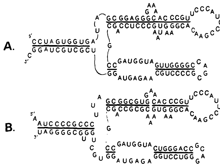
Figure 6: 5S rRNA's from Thermophilic Bacteria. The best complete filtered (12 of 14) solutions for Bacillus stearothermophilus (A) and for Thermus aquaticus (B). No chemical modification or enzymatic cleavage data are available.
