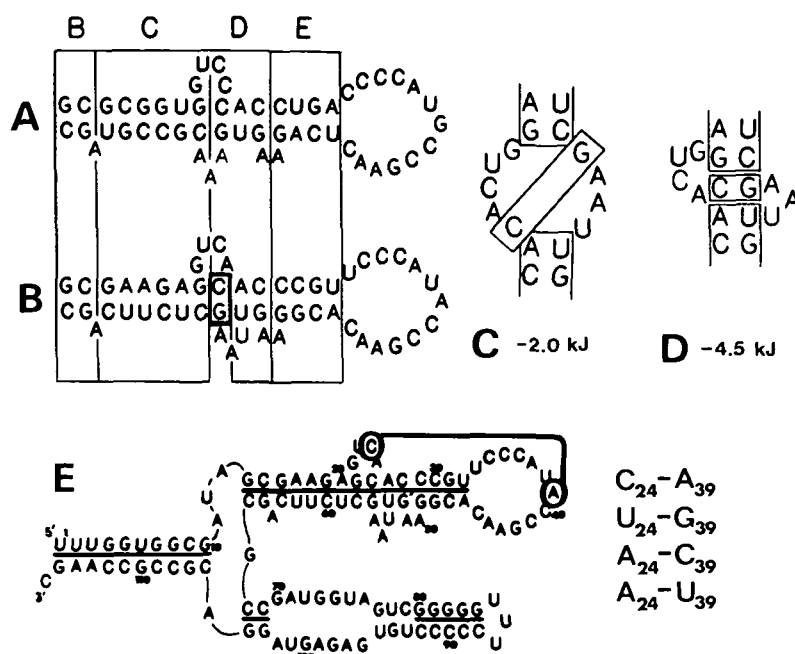
Figure 8: An Intercalated Base Pair. The sequences and secondary structures of the constant length arm are shown for E. coli and B. subtilis , in (A) and (B), respectively. The intercalated C 26 -G 57 pair appears in the helix D region in the B. subtilis sequence. Energy calculations show the energy of the unstacked sequence (C) and intercalated pair (D) and indicate the increased stability of the intercalated pair. The coordinated basepair (E), is shown by a line connecting C 24 and A 39 on the B. subtilis sequence.
