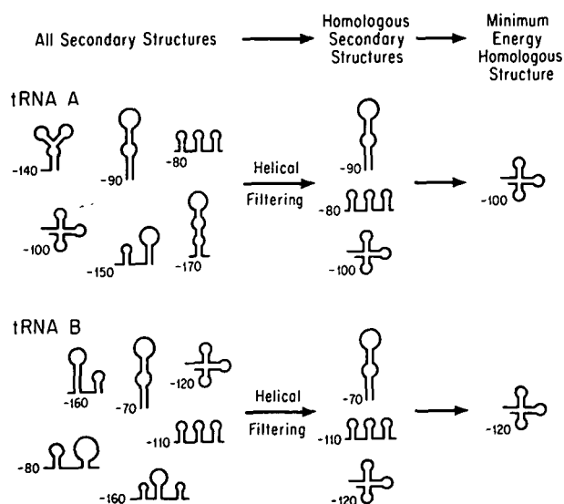
Figure 1: Generalized Scheme for Helical Filtering. A diagrammatic representation of the process of calculating the minimum energy homologous secondary structure is shown using two hypothetical tRNA sequences. In practice, the selection of homologous structures (helical filtering) is done by first accepting homologous helical regions and then using them to construct the sets of common structures. To compare directly entire structures would be prohibitively time consuming.
