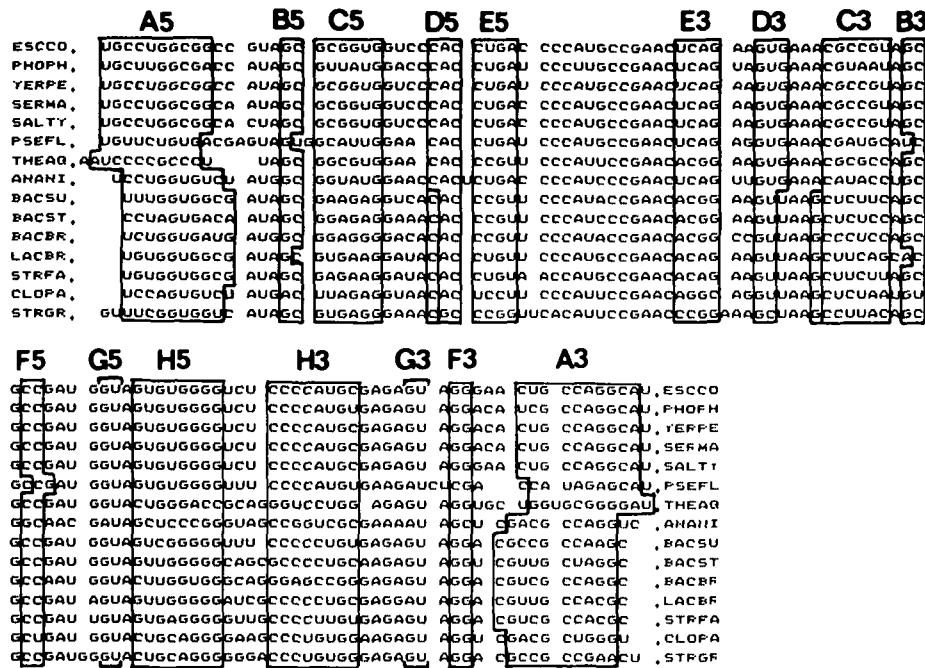
Figure 2: Alignment of Procarvotic 5S rRNA Sequences. Fifteen representative procarvotic 5S rRNAs have been aligned with spaces inserted to maximize the sequence homology. The large numbers denote base numbers of each set of aligned sequences. Spaces between the nucleotides are counted as nonpairing bases. The small numbers are the unspaced nucleotide positions of E. coli 5S rRNA. Since much of the discussion focuses on the E. coli sequence, its numbering system can be used to compare features with those of other species. Each "common" helix appearing in the best filtered structures has also been highlighted by lines in the spaced sequences, to make the degree of universality readily apparent. In Figure 3A each helical region is identified by a letter (A through H), and each halfregion (44) is specified. Thus, B5 is the 5' halfregion of helix B, and B3 is the 3' complementary half-region. Species names have been abbreviated to five letters: ESCCO = Escherichia coli , PHOPH = Photobacterium phosphoreum , YERPE = Yersinia pestis , PSEFL = Pseudomonas fluorescens , THEAQ = Thermus aquaticus , ANANI = Anacystis nidulans , BACSU = Bacillus subtilis , BACST = Bacillus stearothermophilus , BACBR = Bacillus brevis , LACBR = Lactobacillus brevis , STRFA = Streptococcus faecalis , CLOPA = Clostridium pasteurianum , and STRGR = Streptomyces griseus . Original sources of sequences are listed in references 45 and 46 (see also 66), and two minor changes are mentioned in 67.
