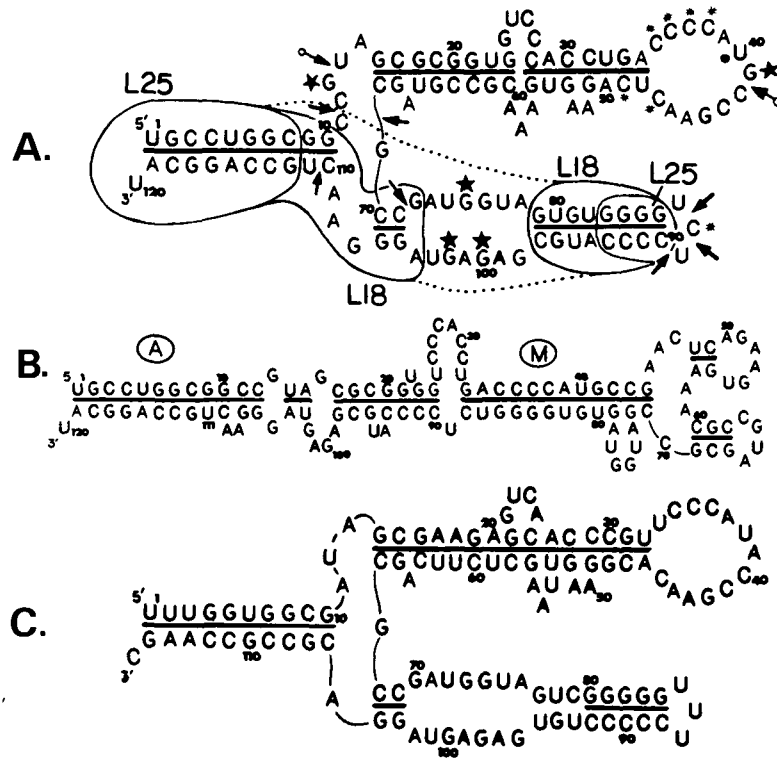
Figure 5: E. coli and B. subtilis 5S rRNAs. The best structure for E. coli (A) and for B. subtilis (C) 5S RNA generated by helical filtering using generated helices common to at least 12 out of 14 of the spaced sequences (in Figure 2). This structure is thought to correspond to the A or native form of 5S RNA. (B) The best computer generated structure of an unfiltered partial solution carried out in four steps, as described in the text. This structure is likely to be related to the B form of E. coli 5S RNA. In (A), (B), and (C), helices are highlighted by lines between the basepairs and are identified by capital letters. Domains of E. coli thought to be protected by ribosomal proteins are enclosed, and sites of chemical modification (★ = kethoxal, ● = carbodiimide, * = methoxamine) and partial enzymatic cleavage (↘ = pancreatic RNase, ↙ = T1 RNase) are indicated in (A) and (B). Base-numbers of some of the nucleotides are shown.
