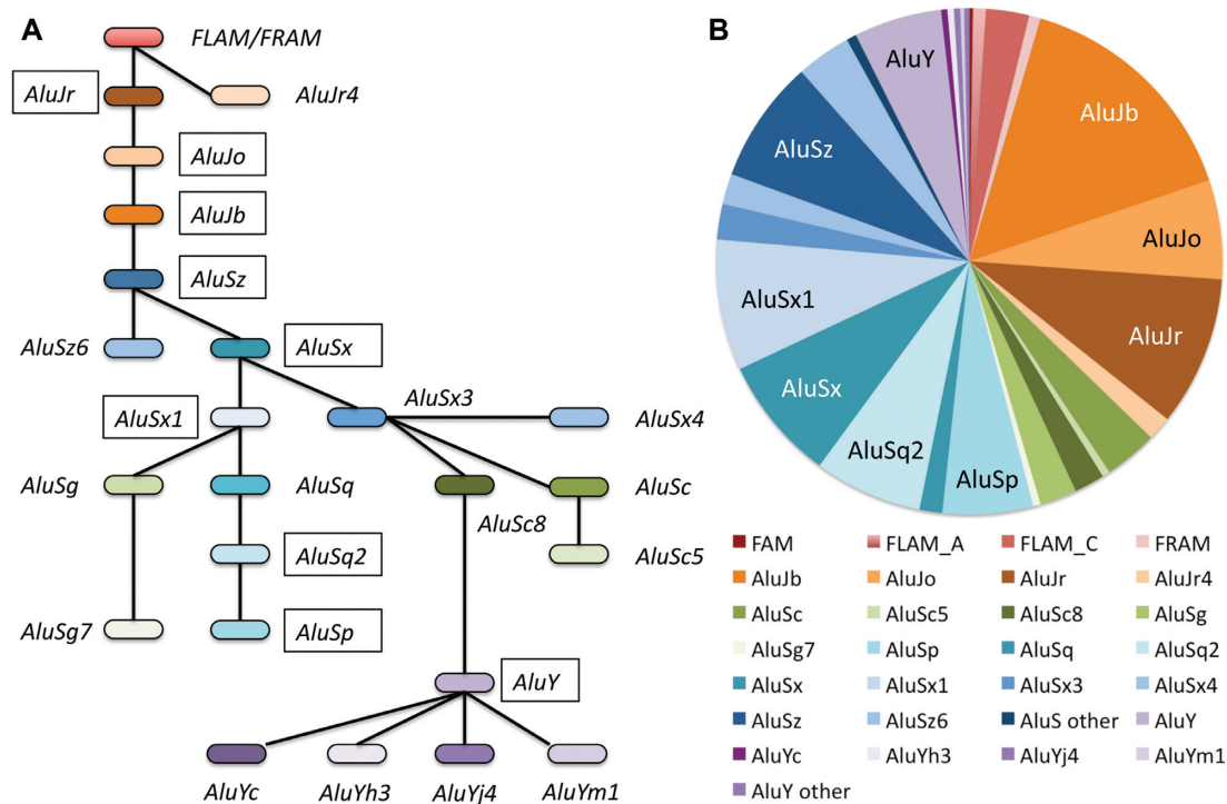
Figure 2. SINE Alu sub-families that overlap coding exons. (A) The SINE Alu family tree based on the family tree in RepeatMasker. The most common sub-families are marked with a black box. (B) The proportion of each Alu sub-family that overlaps coding exons. Members of the FRAM/FLAM, AluJ, AluS and AluY families by their proportion in coding exons in the reference genome. The most common sub-families are labeled in the chart.
