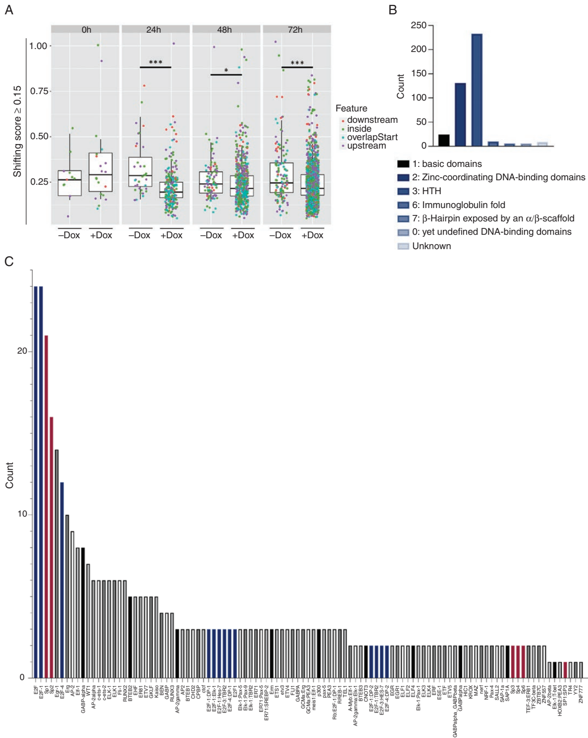
Figure 3. CAGE analysis. (A) Promoter shifting analysis. Boxplots show consensus clusters with a shifting score \geq 0.15 . Significant increase of shifting promoters at timepoints 24, 48, and 72 h after Dox induction. Statistical testing was performed with the Mann–Whitney test: 24 h ( P value: <.0001 (***)), 48 h ( P value: .03 (*)), and 72 h ( P value: .0004 (***)). Shifting promoters were associated with transcriptionally relevant genome annotation features “overlap start” (blue), “inside” (green), “downstream” (orange), “upstream” (violet). X-axis labels: +Dox = dnE47-RFP + Dox versus E47-RFP + Dox; -Dox = dnE47-RFP-Dox versus E47-RFP-Dox. (B and C) TF-binding enrichment analysis after 72 h of those consensus clusters with a shifting score \geq 0.15 showed a time-related increase in TF activity (B), especially for class 1 (basic domains), class 2 (Zinc-coordinating DNA-binding domains), and class 3 (helix-turn-helix domains). An enrichment of specific TF-binding domains was observed for the E2F (C, blue bars) and Sp-family (C, red bars).
