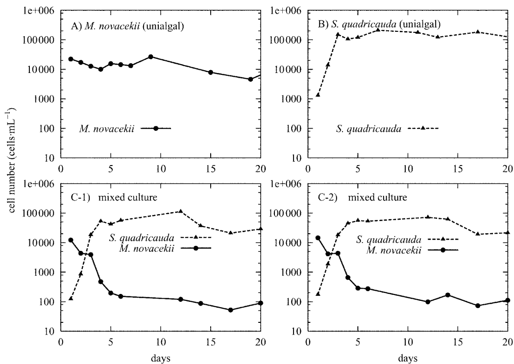
Fig. 2. Growth of M. novacekii and S. quadricauda in chemostat cultures with the dilution rate 0.3 day -1 .
