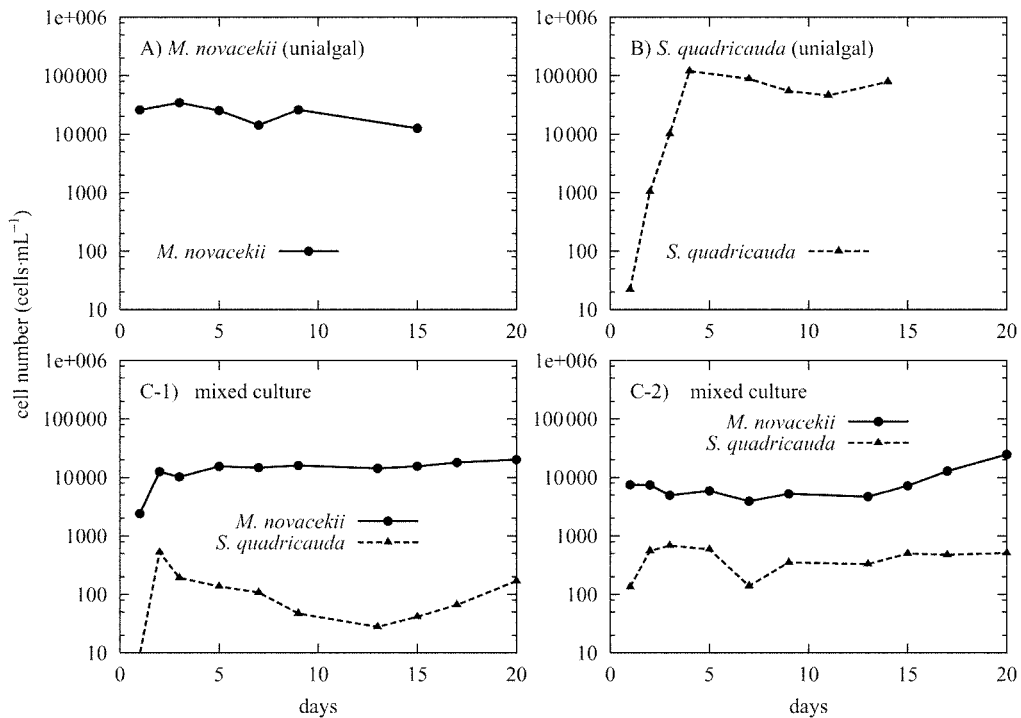
Fig. 1. Growth of M. novacekii and S. quadricauda in chemostat cultures with the dilution rate 0.1 day -1 .
