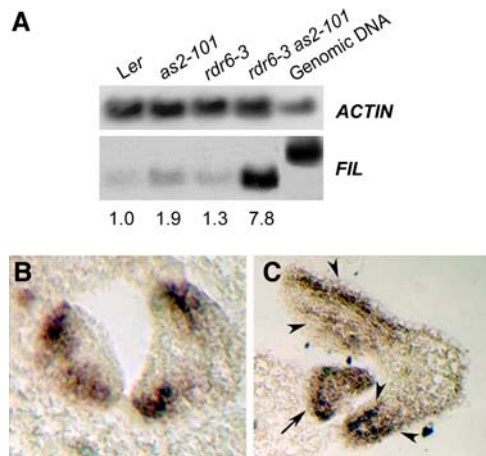
Figure 9. Expression of the FIL Gene.
