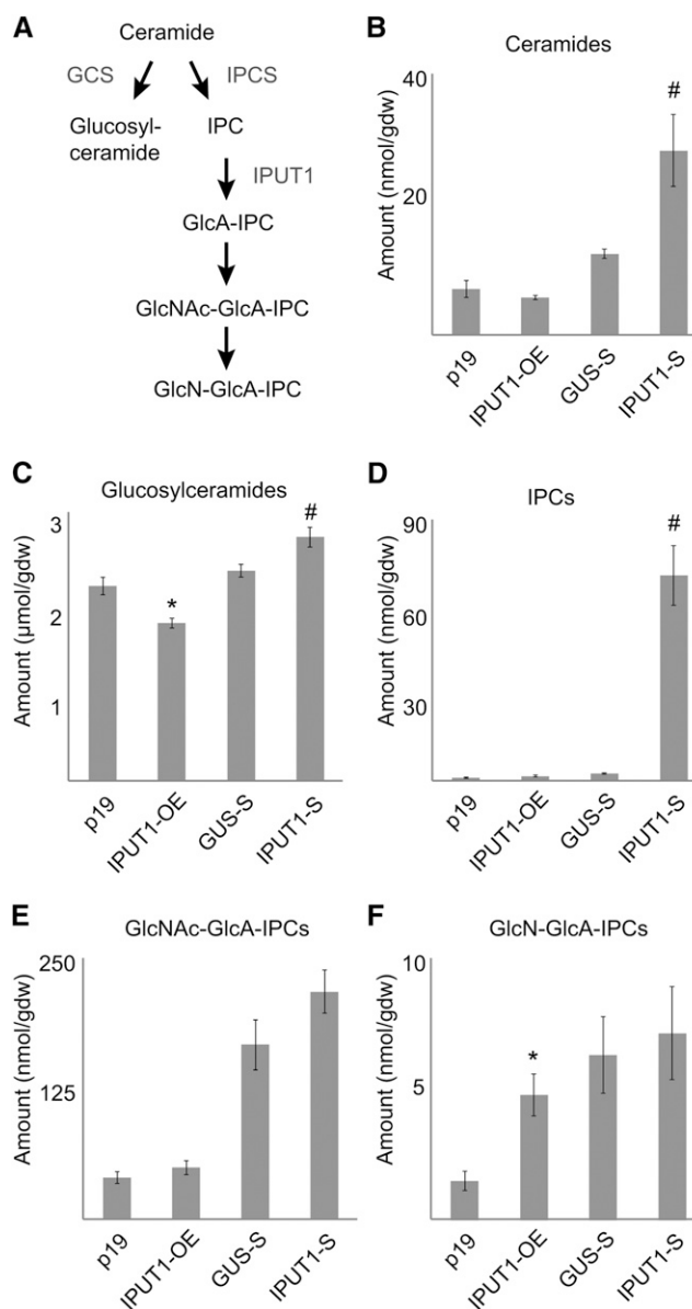
Figure 4. Sphingolipid Profiles in N. benthamiana Plants with Altered Expression of IPUT1 .
