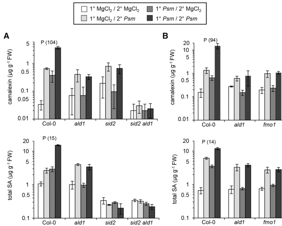
Figure 7. SAR-Associated Priming of Camalexin and SA Biosyntheses Requires a Functional Pip/FMO1 Module, and SAR Priming of Camalexin Production Is SA Dependent.
