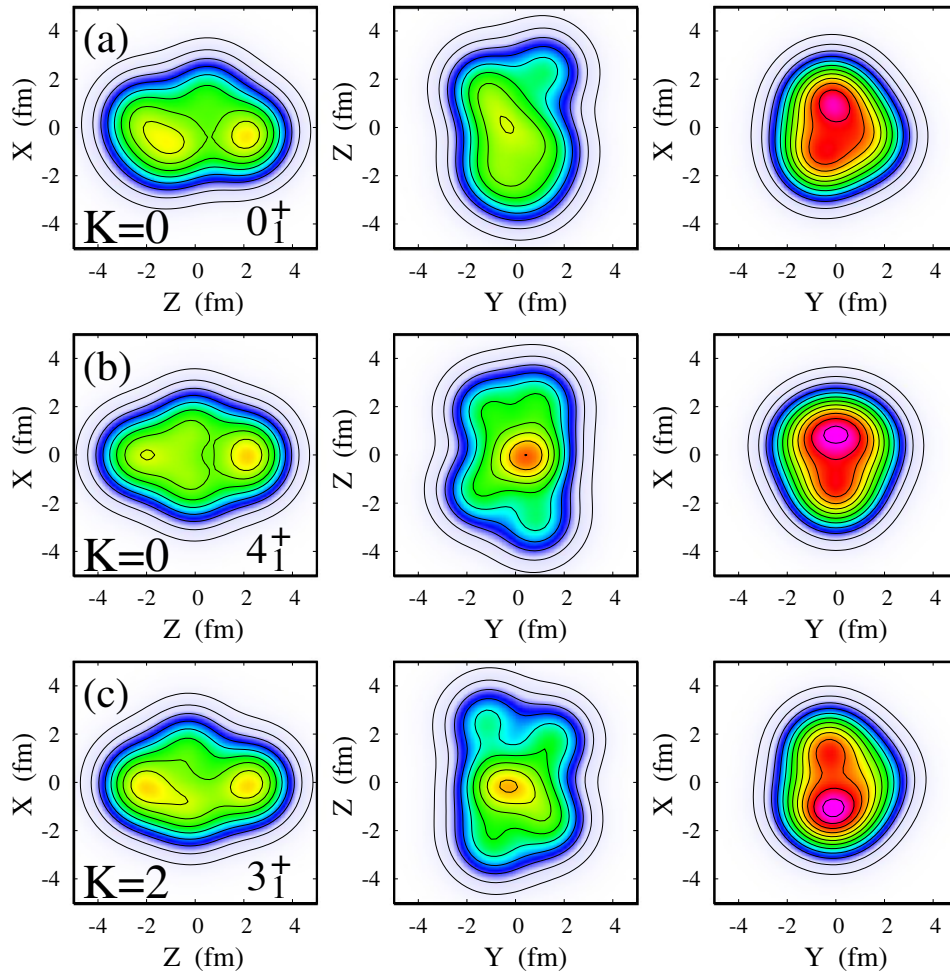
Fig. 1. Density distribution of the intrinsic wave functions before the parity and total angular momentum projections of the 0_1^+(K^\pi = 0^+) , 4_1^+(K^\pi = 0^+) , and 3_1^+(K^\pi = 2^+) states obtained by VAP. In the left, middle, and right panels, the densities are projected onto the X - Z , Y - Z , and Y - X planes by integrating along the Y , X , and Z axes, respectively. The intrinsic axes are selected as the principal axes in the following order: \langle ZZ \rangle \geq \langle YY \rangle \geq \langle XX \rangle .
