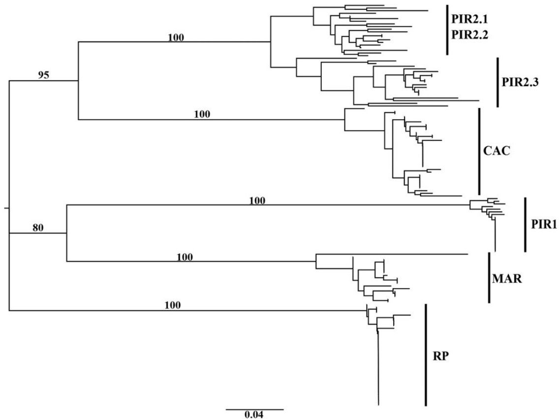
Figure 3. Dendrogram obtained with the neighbour-joining algorithm, based on Jaccard dissimilarity for five populations [Ribeirão Preto/SP (RP), Cáceres/MT (CAC), Piracicaba1/SP (PIR1), Piracicaba2/SP (PIR2.1, PIR2.2, PIR2.3) and Maringá/PR (MAR)] of Oeceoclades maculata .
