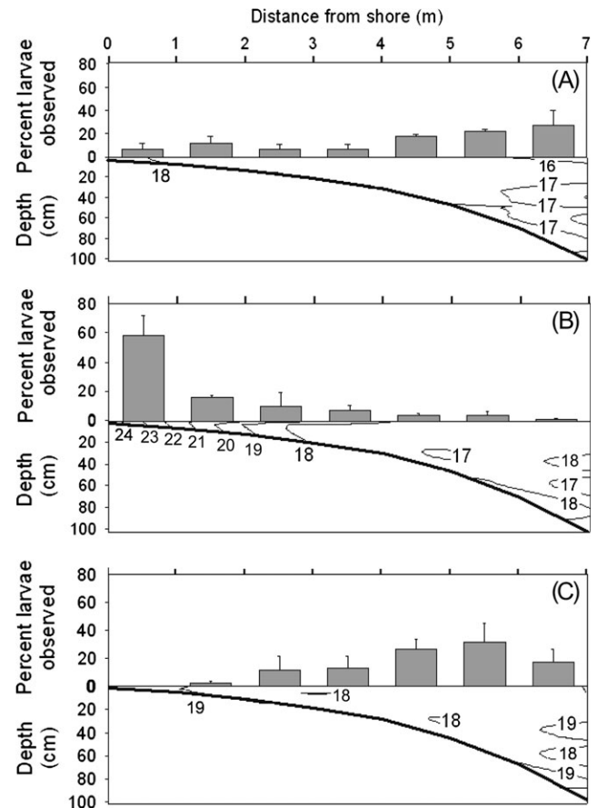
Figure 3 Distribution of Bufo boreas larvae in Todd Lake, Deschutes County, OR, on 10 August 2006. The thick black line indicates the bottom of the lake. Contour lines represent thermal stratification in degrees Celsius. Bars indicate the mean percentage ( \pm SE) of B. boreas tadpoles observed in 3 transects in the morning (A), midday (B), and evening (C).
