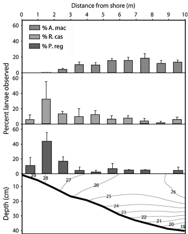
Figure 2 Distribution of the larvae of 3 species at midday on 20 July 2006 in Susan's pond, Deschutes County, OR. Thick black line in the bottom panel represents the bottom of the pond, and the numbers are temperature in degrees Celsius. Bars represent the mean percentage of larvae of each species observed at each depth \pm standard error (mean of 3 transects). The majority of anuran larvae ( Rana cascadae and Pseudacris regilla ) were observed closer to shore in water <15 cm deep. Most salamander larvae ( Ambystoma macrodactylum ) were observed in water >20 cm deep.
