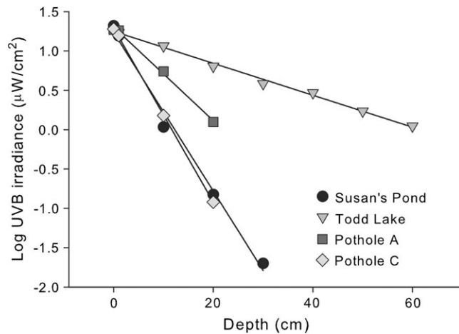
Figure 1 UVB profiles from all sites during midday. Todd Lake had the highest UVB transmittance. Only ponds A and C are shown from the potholes for clarity. The transmittance of pond B was nearly identical to pond A, whereas pond D was similar to pond C. Note the log scale used on the y axis.
