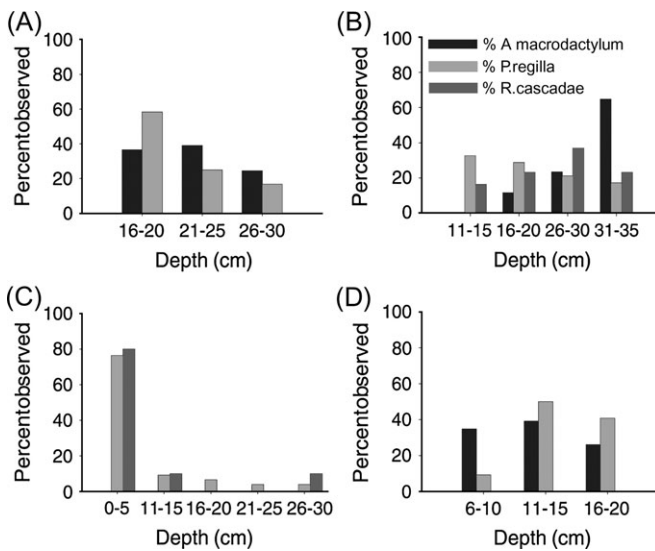
Figure 4 Distribution of larvae at midday on 10 August 2006 at the potholes, Deschutes County, OR. Individual potholes (A–D) are shown separately. Bars indicate percentage of each species observed within each depth class.
