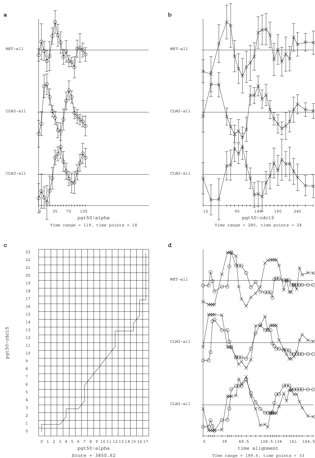
Fig. 2. Overall genewarp alignment of alpha and cdc15 series using large set pgt50 of differentially expressed genes. This alignment is more stable than those of smaller sets of genes or genes that are less differentially expressed (see text). (a) Average trajectories of MET, CLB2, and CLN2 clusters of genes in input pgt50:alpha data series. Error bars represent standard deviations at each time point. (b) Average trajectories with error bars of the same clusters in pgt50:cdc15 series. (c) Path graph and optimal path based on entire set of 990 genes in the input data. (d) Time alignment of the MET, CLB2, and CLN2 clusters based on (c).
