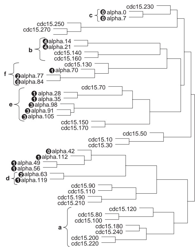
Fig. 3. Results of clustering of alpha and cdc15 time points based on the pgt50 set of genes and comparison of time point clusters with time warping alignments of pgt50:alpha versus pgt50:cdc15 (see Figure 2) and the alignments of pgt50:alpha and pgt50:cdc15 half series (see text and web supplement). Groupings a–f and time point labels 0–4 are described in the text.
