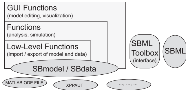
Fig. 1. Modular structure of the toolbox. The toolbox is designed in a modular way. Optionally, freely available third party software packages are used, e.g. to (i) perform bifurcation analysis and (ii) realize an interface to SBML.
