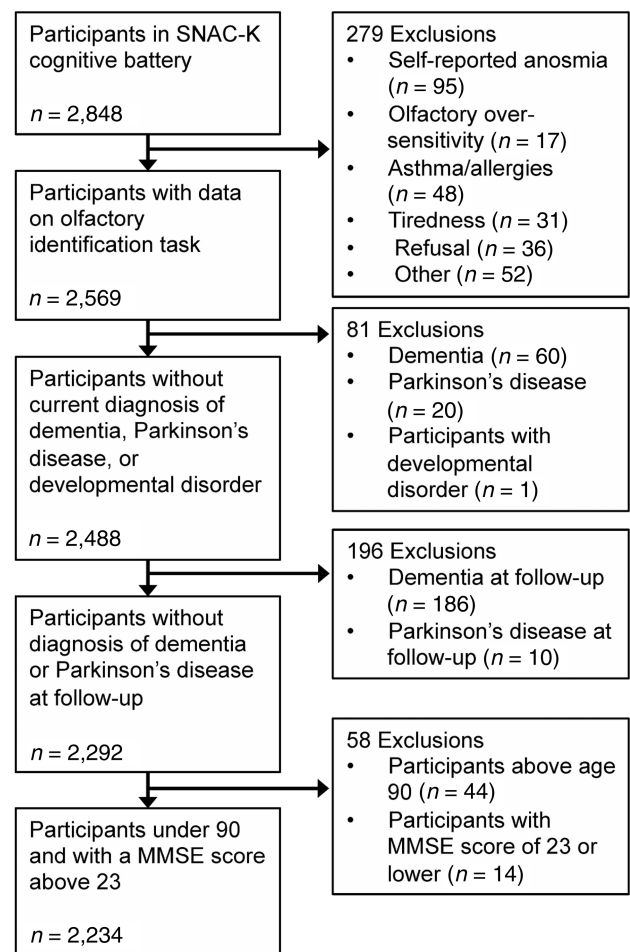
Figure 1. Exclusion flowchart.
