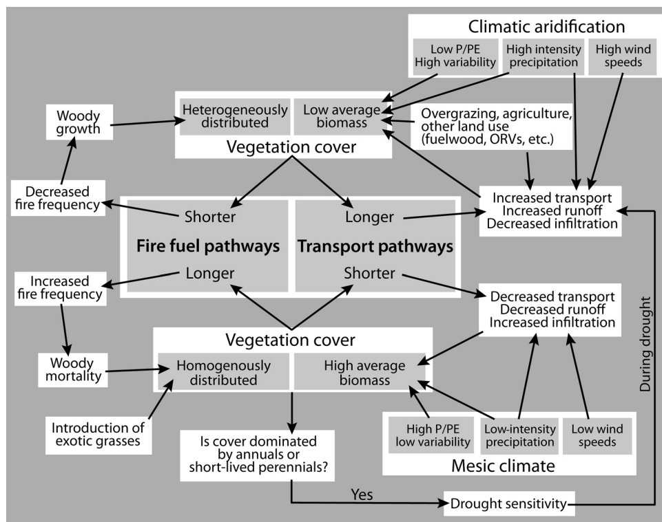
Figure 2. A model of desertification linking the length of the connected pathway, or LOCOP, to climate change, land use, and vegetation cover. Abbreviations: ORVs, off-road vehicles; P/PE, precipitation/potential evapotranspiration.
