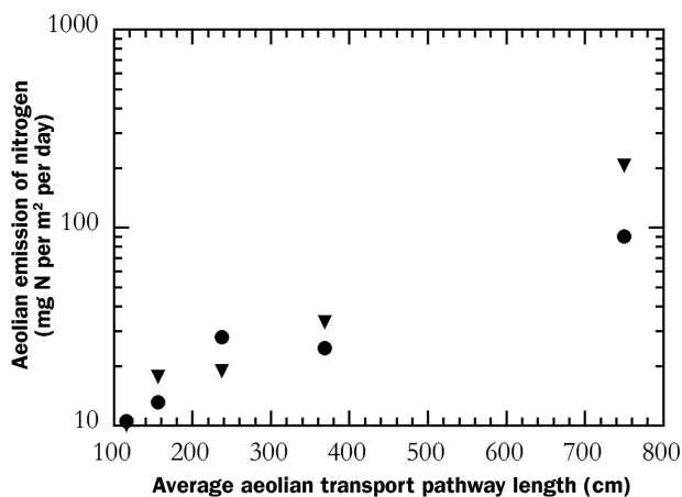
Figure 3. The emission of nitrogen (in milligrams of nitrogen per square meter per day) on dust from experimental plots in the Jornada Experimental Range, New Mexico, versus the length of the average aeolian transport pathway, in centimeters. Source: Based on data from Li FR and colleagues (2005) for spring (triangles) and summer (circles) of 2005.
