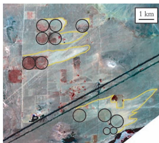
Figure 4. AVIRIS (Airborne Visible/Infrared Imaging Spectrometer) image (NIR:Green:Blue::R:G:B) of abandoned central-pivot agricultural fields in the Mojave Desert (black circles). Areas of wind-blown sand leading to expanding desertification are outlined in yellow. Source: Adapted from Okin and colleagues (2001).
