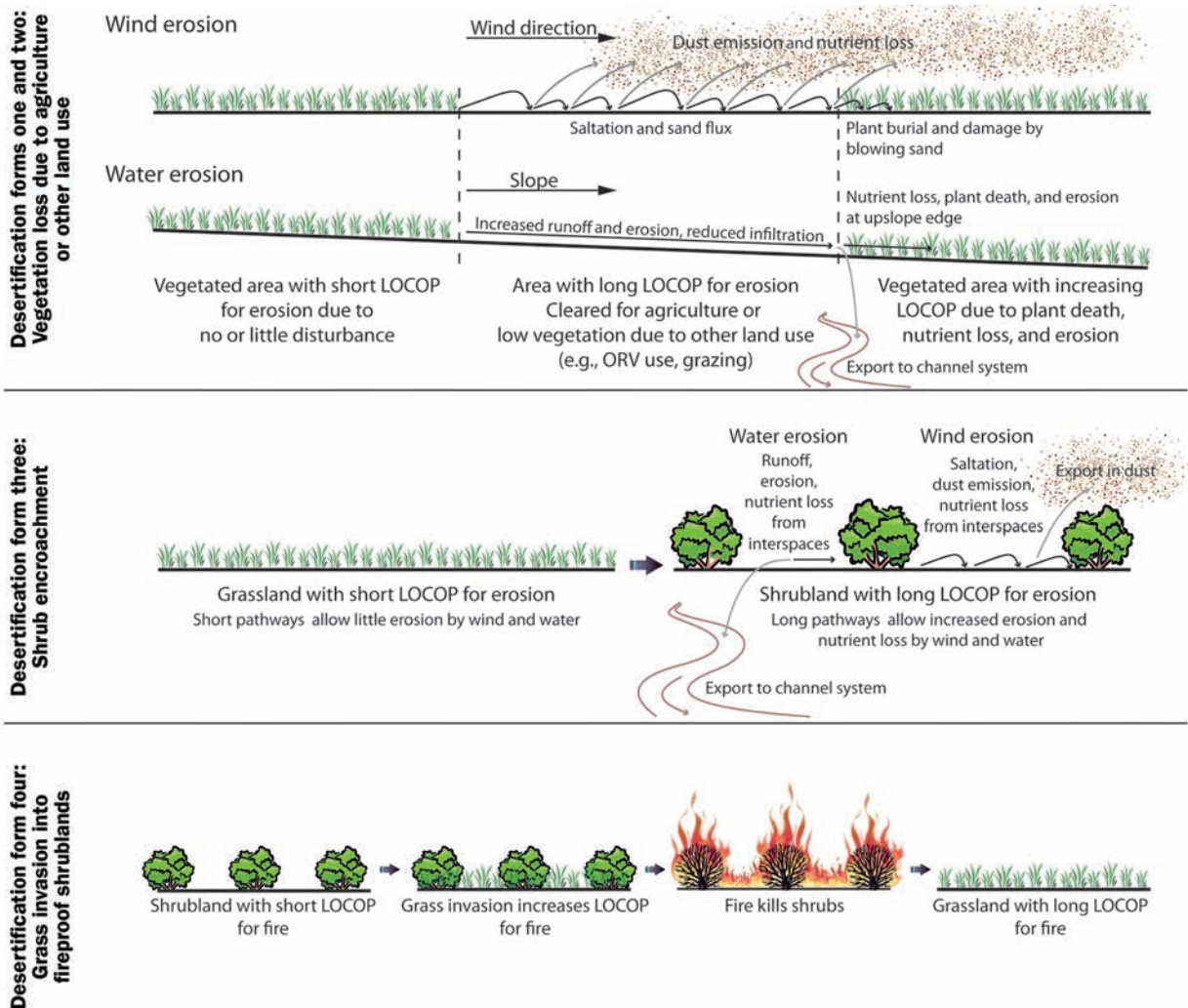
Figure 1. Schematic representation of the four forms of desertification and feedback processes that can be explained by changes in connectivity. Abbreviation: LOCOP, length of the connected pathway; ORV, off-road vehicle.
