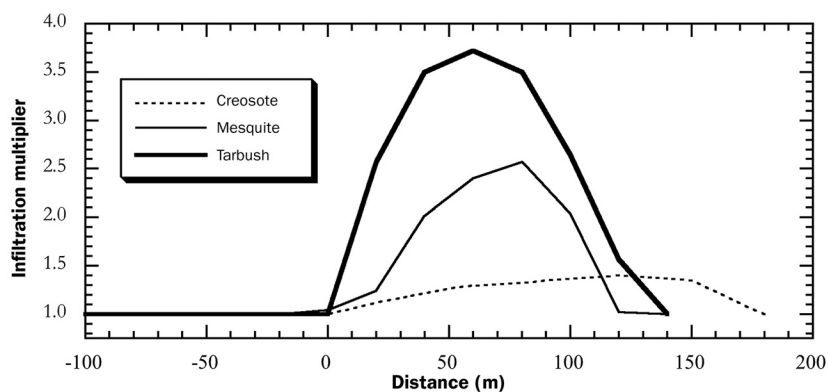
Figure 5. Relative infiltration of water flowing downslope from three shrublands (negative distances) into grasslands (positive distances), with the grass-shrub boundary at distance = 0 meters. The infiltration multiplier at a point is the infiltration rate at that point divided by the infiltration in the high-connectivity shrubland. Water infiltrates preferentially (e.g., infiltration multiplier > 1) in low-connectivity grasslands downslope of high-connectivity shrublands, which contribute runoff (e.g., infiltration multiplier is approximately 1). Source: Adapted from data in Mueller and colleagues (2007b).
