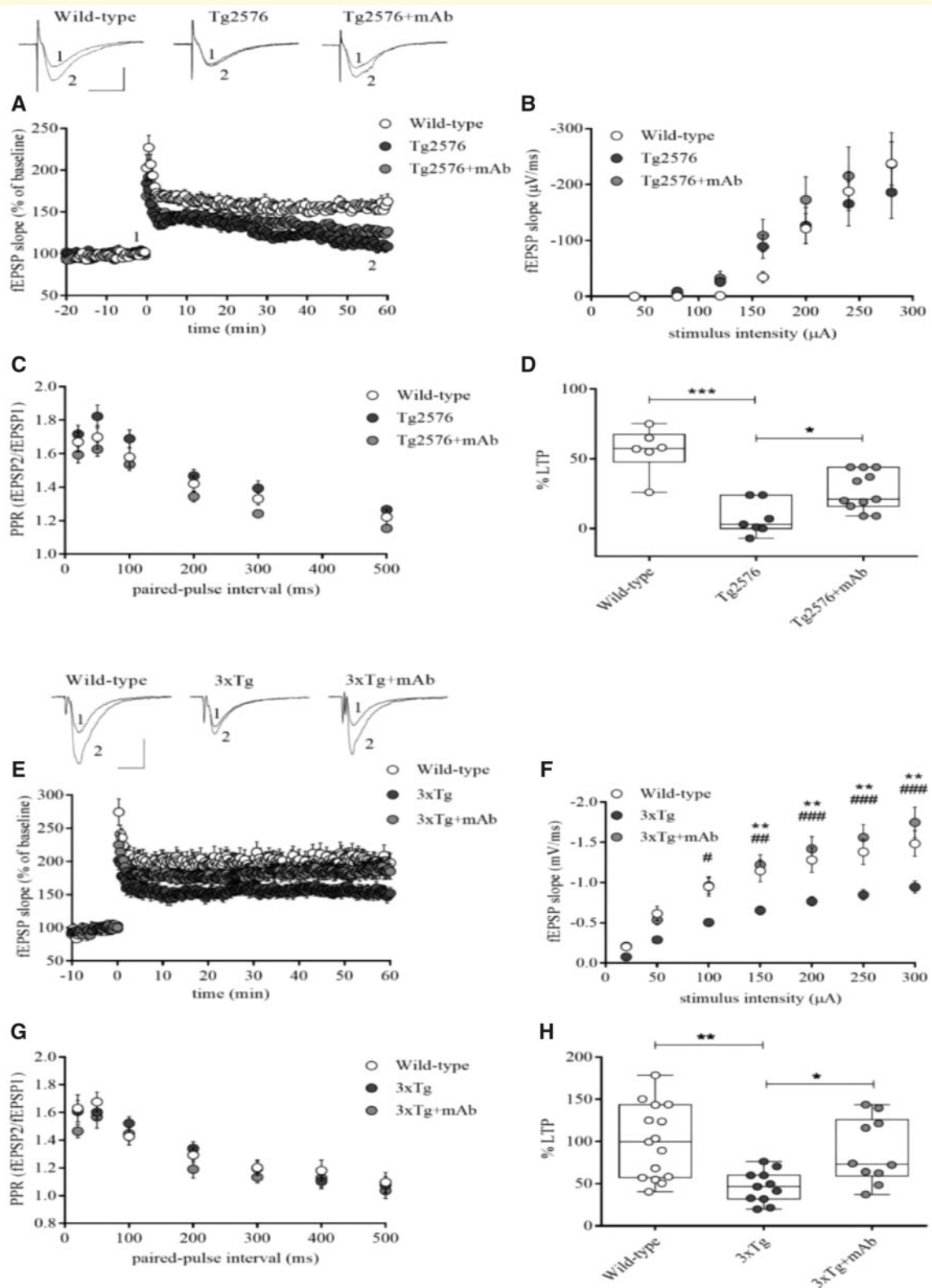
Figure 7 Reduction of cognitive deficits in 12A12mAb-immunized Tg-Alzheimer's disease mice correlates with an increased LTP. (A, D) For Tg2576; (E, H) for 3xTg time plot of average fEPSP responses (A, E) and changes in magnitude of LTP at CA3-Ca1 synapses (D, H) were calculated among animals ( n = 6-10 ) from three experimental groups (WT, Tg-Alzheimer's disease and Tg-Alzheimer's disease + mAb) of both strains. At least seven slices from six different mice were recorded for each experimental condition. Data are presented as the mean ( \pm SEM). The traces above the plot show fEPSPs at baseline (1) and at 60 min after LTP induction (2). The box-whisker plots show pooled data. Statistically significant differences (see details in the main text) were calculated by ANOVA followed by post hoc test for multiple comparisons among more than two groups. P < 0.05 was accepted as statistically significant (* P < 0.05 ; ** P < 0.01 ; *** P < 0.0005 ;
