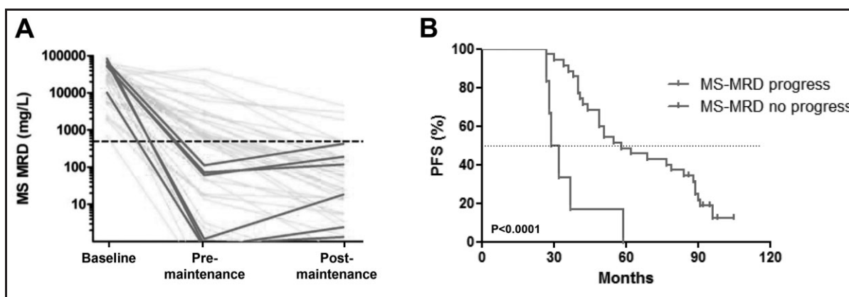
Fig. 3. MS-MRD monitoring.
