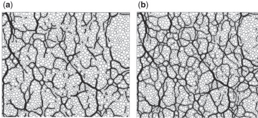
FIG. 20. The contacts and forces in a granular network at two different force thresholds. (a) When only contacts with forces f > 1.3\langle f \rangle (where \langle f \rangle is the mean force) are included, the resulting network is composed of many disconnected components. (b) As one decreases the threshold, the components grow, and if only contacts with f > \langle f \rangle are included, the network is connected and ‘percolates’ along the axis of compression. The system is a numerical simulation of a dense, 2D collection of hard spheres under biaxial compression. We adapted this figure, with permission, from [19].
