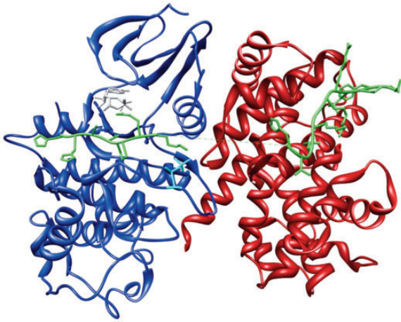
Figure 3. The Cyclin A-Cdk2-Cdc6 complex. Crystal structure of Cdc6 peptide bound to the active Cyclin A-Cdk2 complex (PDB:2CCI) (71), showing Cdc6 (green), Cyclin A (red) and Cdk2 (blue) phosphorylated at T160 (cyan) and bound with the ATP analogue Adenylyl Imidodiphosphate (AMPPNP) (grey). This figure was generated using UCSF Chimera (83).
