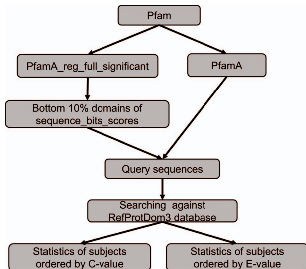
Figure 5. The benchmarking method to compare the performance between PSISearch2D and the original PSISearch2.
