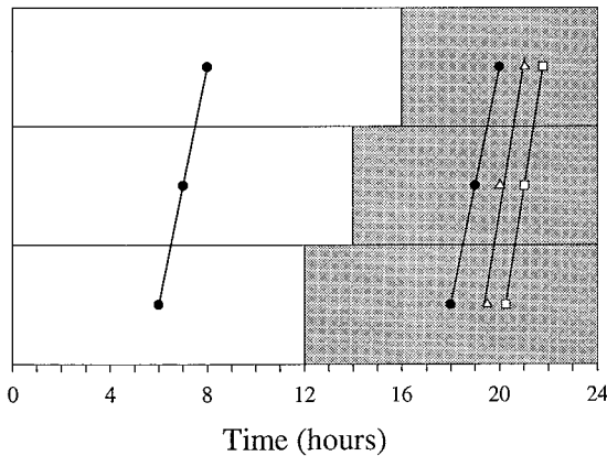
Fig. 1. Onset (triangles) and mean (squares) times of calling of Agrotis ipsilon virgin females reared under three photoregime conditions (white bar = photophase, gray bar = scotophase; 12:12, 14:10, and 16:8 [L: D] h) in relation to lights-on, lights-off, mid-photophase (black dots on white area), and mid-scotophase (black dots on gray area).
