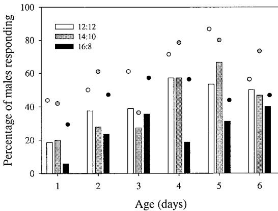
Fig. 2. Percentages of oriented upwind flight (dots) and contact (bars) with a synthetic pheromone blend source (Z7-12: Ac, Z9-14: Ac, and Z11-16: Ac, 3:1: 6 \mu g) in a wind tunnel bioassay by 1- to 6-d-old Agrotis ipsilon males reared under three photoregime conditions ( n = 11-20 ). White: 12:12 (L:D) h, gray: 14:10 (L:D) h, black: 16:8 (L:D) h.
