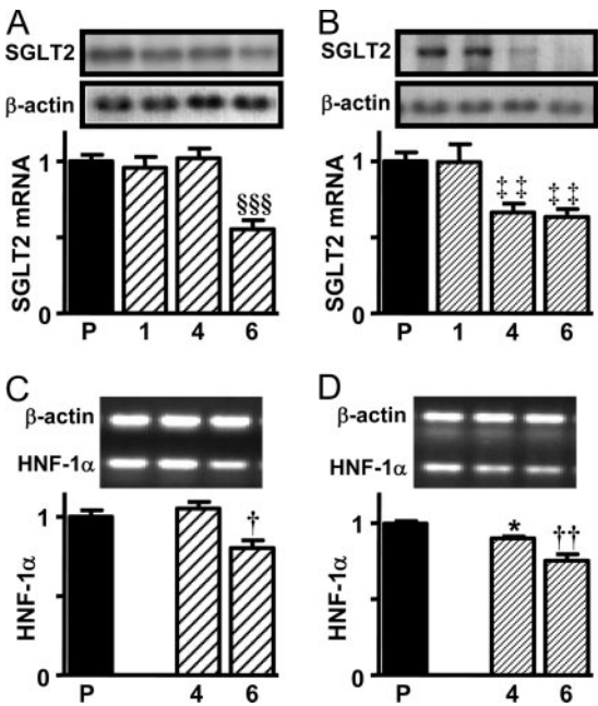
FIG. 3. SGLT2 (A and B) and HNF-1α (C and D) mRNA analysis in renal cortex of diabetic rats submitted to short-term treatment with insulin (A and C) or phlorizin (B and D). Diabetic rats were studied after 1, 4, and 6 d of treatment with insulin or phlorizin. Placebo treatment (P) was saline for insulin study and propylene glycol for phlorizin treatment. One-, 4- and 6-d data of each placebo treatment were pooled. A and B, SGLT2 mRNA analysis performed by Northern blotting of poly(A) RNA: at the top, typical images of the SGLT2 and respective β-actin mRNAs, at the bottom, the abundance of the SGLT2 mRNA normalized to β-actin. C and D, HNF-1α mRNA analysis performed by RT-PCR: at the top, typical images of the HNF-1α and respective β-actin amplicons, at the bottom, the estimated abundance of the HNF-1α mRNA normalized to β-actin. Data are mean ± SEM of six and five animals in each group, respectively, for SGLT2 and HNF-1α analysis, evaluated in three different experiments. *, P < 0.05 vs. P (placebo); †, P < 0.05 ; ††, P < 0.01 vs. P (placebo) and 4 d; †††, P < 0.01 vs. P (placebo) and 1 d; §§§, P < 0.001 vs. all groups; ANOVA, Student-Newman-Keuls.
