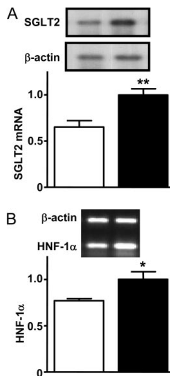
FIG. 1. SGLT2 (A) and HNF-1 \alpha (B) mRNA analysis in renal cortex of nondiabetic (open bars) and diabetic (closed bars) rats. A, SGLT2 mRNA analysis performed by Northern blotting of poly(A) RNA: at the top, typical images of the SGLT2 and respective \beta -actin mRNAs, at the bottom, the abundance of the SGLT2 mRNA normalized to \beta -actin. B, HNF-1 \alpha mRNA analysis performed by RT-PCR: at the top, typical images of the HNF-1 \alpha and respective \beta -actin amplicons, at the bottom, the estimated abundance of the HNF-1 \alpha mRNA normalized to \beta -actin value. Data are mean \pm SEM of five animals in each group, evaluated in three different experiments. *, P < 0.05 ; **, P < 0.01 vs. nondiabetic rats; Student's t test.
