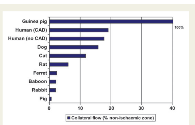
Figure 3 Inter-species differences in coronary collateral relative to normal flow in the non-occluded vessel.
