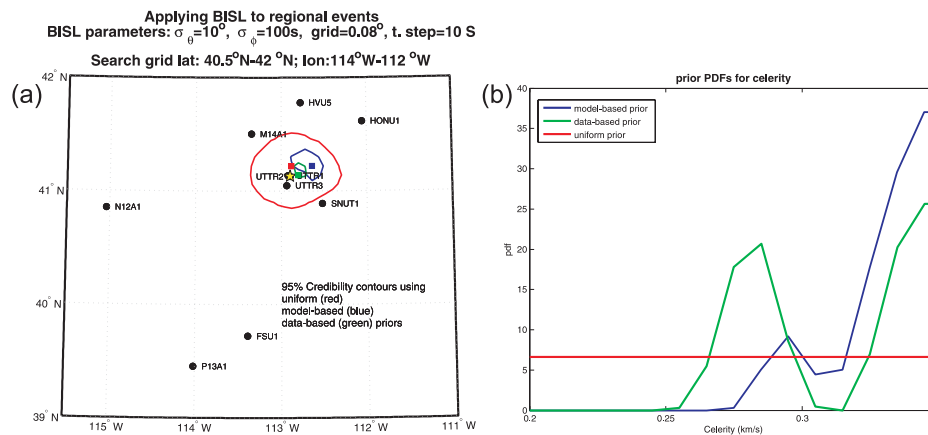
Figure 10. Locating the 2007 August 6 UTTR event using the BJSL technique and three different network-average prior pdfs, uniform, model CRH-based and data CRH-based. (a) Temporary infrasound network location map (black dots), 95 per cent credibility contours using uniform (red), model CRH-based (blue) and data CRH-based (green) priors, with their maximum a posteriori (MAP) points shown as squares. Ground truth (yellow star). (b) Prior pdfs corresponding to the MAP point for the event location. Uniform (red), model CRH-based (blue) and data CRH-based (green).
