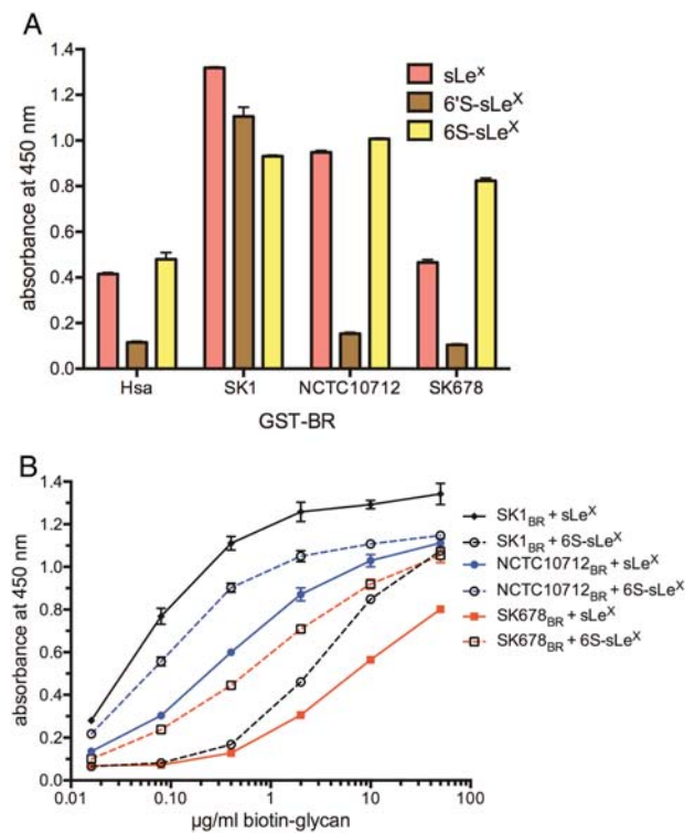
Fig. 10. Binding of the Hsa-like BRs to sulfated forms of sialyl Lewis X. (A) Binding of biotinylated sLe x , 6'S-sLe x or 6S-sLe x (10 \mu g/mL) to immobilized GST-BRs. Binding is reported as the mean \pm standard deviation, with n = 3 . (B) Binding of biotinylated sLe x or 6S-sLe x to immobilized GST-BRs. Binding is reported as the mean \pm standard deviation, with n = 2 . This figure is available in black and white in print and in color at Glycobiology online.
