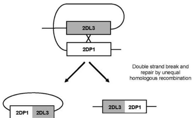
Figure 10. Proposed mechanism behind the formation of the KIR2DL3/2DP1 gene; deletion of ~17 kb by homologous unequal intra-chromosomal recombination (Alu-mediated). A DNA break is introduced at the recombination hotspot site of an Alu repeat within a KIR gene. A second break occurs 17 kb away that contains sequence homologous to the first break site. The two homologous sequences serve as a substrate for double-strand break repair, which leads to deletion of the intervening sequences between the break sites.
