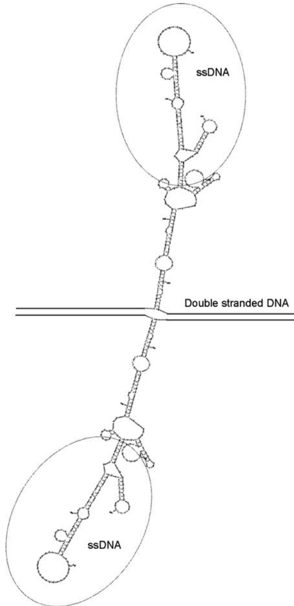
Figure 12. Potential ssDNA conformation formed from the MLT1 sequence at the KIR2DS1 breakpoint region. The breakpoint interval sequences are circled. Such protrusive non-B DNA structures may catalyse KIR rearrangements.
