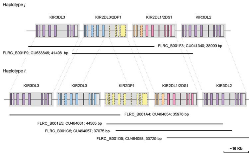
Figure 3. Gene annotation of the sequenced portions of the j and t haplotypes. Locations of fosmid clone insert sequences are shown below each haplotype.
