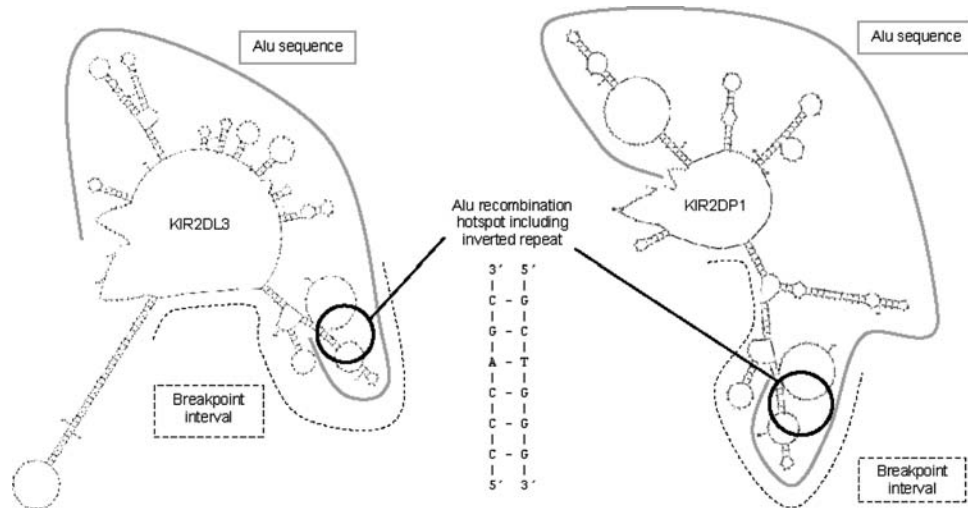
Figure 9. Potential ssDNA secondary structures formed at the KIR2DL3 (left) and KIR2DP1 (right) breakpoint regions ssDNA. These structures can serve as recognition signals to induce strand breaks that cause genomic rearrangements by recombination-repair. The dashed line indicates the breakpoint intervals. The solid grey line depicts the full ~282 bp Alu sequence. The black circle contains the core 22 nucleotides of the Alu recombination hotspot (5'-TGTAATCCCAGCACTTTGGGAG-3').
