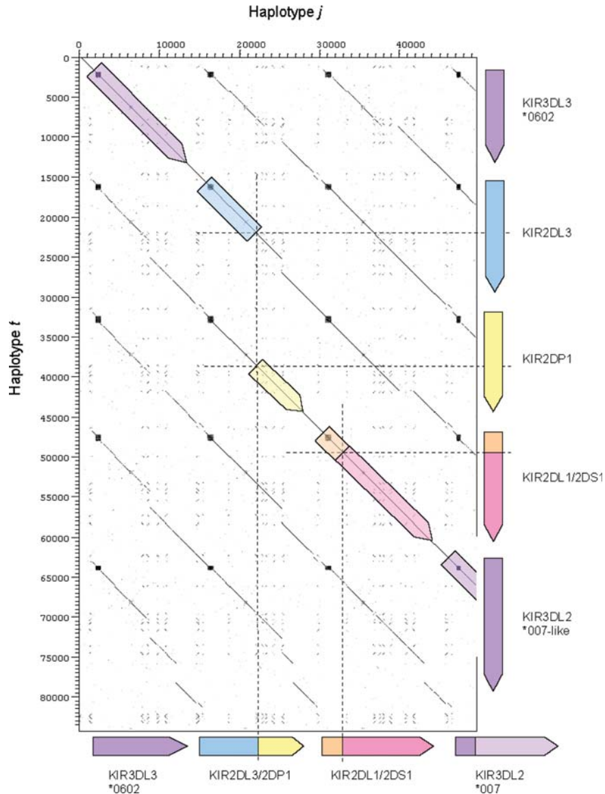
Figure 6. Dot matrix analysis of the j and t KIR haplotype sequences. The plot shows the four KIR genes of the j haplotype on the x -axis and the 5 KIR genes of the t haplotype on the y -axis. Regions of similarity are identified as a concentration of dots forming diagonal lines. Minisatellites can be visualized as boxes. The deletion breakpoints on both haplotypes are indicated by dashed lines. The intergenic regions and introns of the KIR loci are well conserved.
