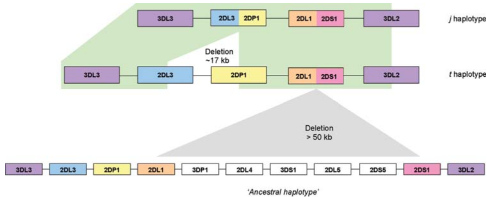
Figure 7. The presumed order of genomic deletions in the formation of the j haplotype. First, a > 50 kb deletion fused the KIR2DL1 and KIR2DS1 genes creating the KIR2DL1/DS1 hybrid gene. Subsequently, a smaller ~17 kb deletion fused the KIR2DL3 and KIR2DP1 genes to form the KIR2DL3/2DP1 gene. A representative KIR ‘B’ haplotype is shown below the deletion haplotypes as an example of one potential ancestral haplotype involved in the derivation of haplotype t . The represented haplotype was the most frequent observed in a panel of 85 Caucasoid individuals with a frequency of 0.124 (41). Apart from the ~17 kb deletion and a single nucleotide, the j and t haplotype sequences are identical, raising the possibility of intra-chromosomal recombination in the formation of the j haplotype, and implicating the t haplotype as the single precursor of the j haplotype.
