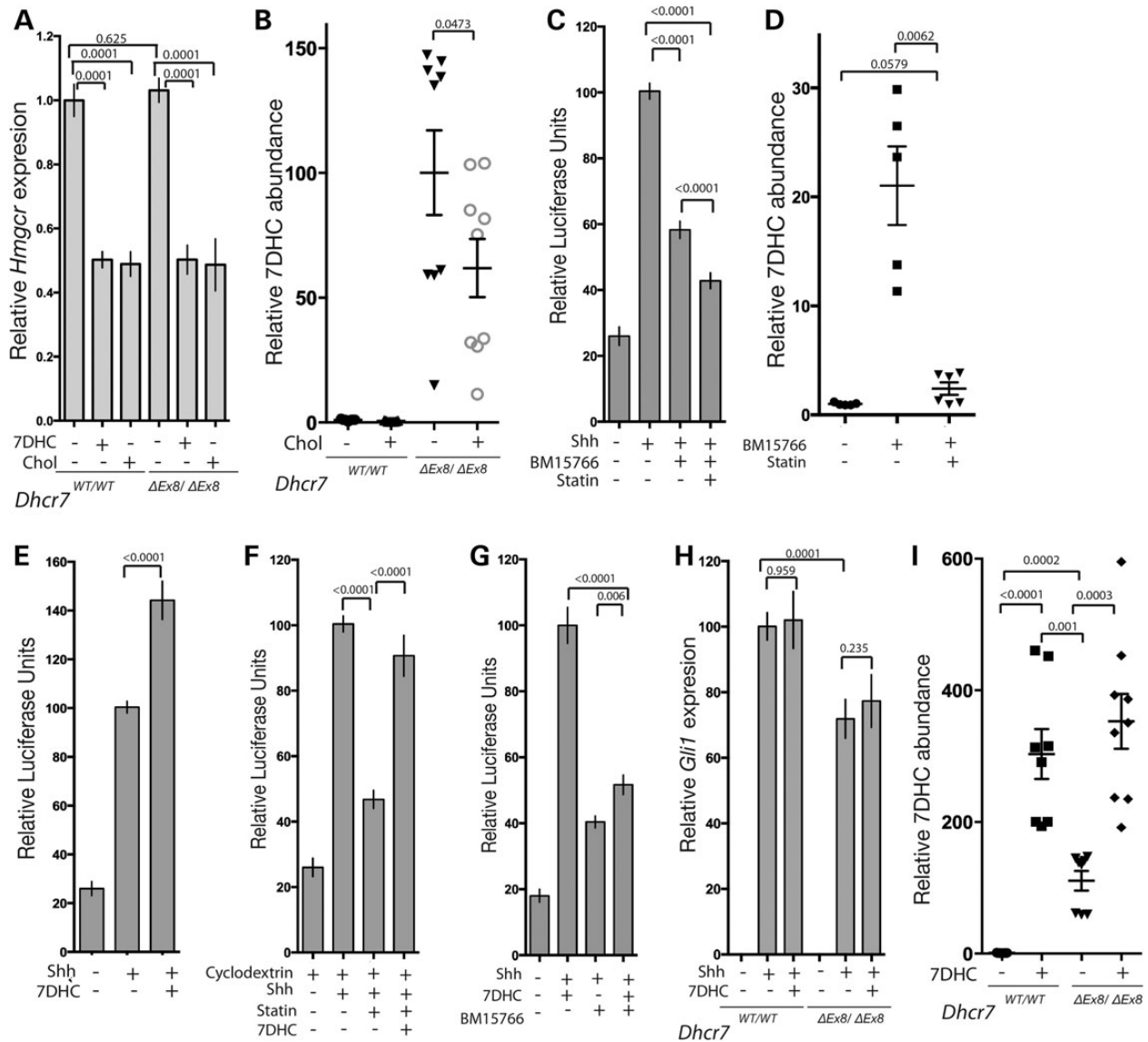
Figure 5. 7DHC accumulation does not inhibit SHH signaling. (A) Hmgcr expression measured by qPCR is equivalent in WT and Dchr7 \Delta Ex8/\Delta Ex8 MEFs, and reduced by 7DHC and cholesterol (n = 5). (B) Exogenous cholesterol reduces the elevated 7DHC levels in Dchr7 \Delta Ex8/\Delta Ex8 MEFs. Abundances determined by GC-MS. P-values are from paired t-tests. (C) Inhibition of SHH-induced GLI-reporter activation by BM15.766 in Shh-LIGHT2 cells is not reversed by Lovastatin (n = 20). (D) Lovastatin blocks 7DHC accumulation in 3T3 cells treated with BM15.766. (E) 7DHC did not inhibit SHH-induced GLI-reporter activation (n = 20). (F) 7DHC rescued reduced GLI-reporter activation by SHH in the presence of 5 \mu M Lovastatin and 0.1% 2-hydroxypropyl- \beta -cyclodextrin (n = 16). (G) 7DHC did not potentiate the inhibitory effect of BM15.766 on SHH-induced GLI-reporter activation (n = 20). (H) 7DHC had no effect on the Gli1 transcriptional response of SHH stimulated Dchr7 \Delta Ex8/\Delta Ex8 or WT MEFs. Paired t-test (n = 9). (I) Exogenous 7DHC accumulates in WT and Dchr7 \Delta Ex8/\Delta Ex8 MEFs. P-values are from paired t-tests. All panels illustrate mean \pm SEM. P-values are from Mann-Whitney tests unless stated otherwise.
