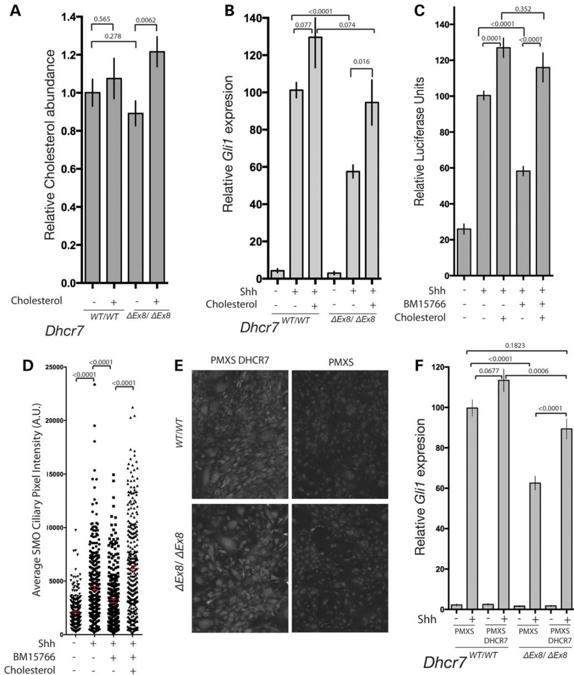
Figure 4. DHCR7 cholesterol biosynthetic activity is required for normal SHH signalling. (A) Addition of exogenous cholesterol raised cellular cholesterol levels of Dhc7^{\Delta Ex8/\Delta Ex8} MEFs as determined by GC-MS. (B) Gli1 transcriptional response of SHH stimulated WT and Dhc7^{\Delta Ex8/\Delta Ex8} MEFs cultured with or without additional cholesterol. Mean \pm SEM. P-values from paired t-tests ( n = 10 ). (C) Inhibition of GLI-reporter activation by BM15.766 in Shh-LIGHT2 cells cultured with or without additional cholesterol. Mean \pm SEM. P-values from the Mann-Whitney test ( n = 20 ). (D) The mean pixel value of individual SMO immunostained cilia was reduced in SHH-stimulated NIH3T3 fibroblasts cultured with BM15.766. The effect was reversed by cholesterol. Mean \pm SEM. P-values from the Kolmogorov-Smirnov test. (E) Immunofluorescence staining of human DHCR7 overexpressed in MEFs by retroviral transduction compared with untransfected control MEFs. (F) DHCR7 overexpression rescued the reduced Gli1 transcriptional response of SHH stimulated Dhc7^{\Delta Ex8/\Delta Ex8} MEFs. Mean \pm SEM ( n = 16 ). P-values from paired t-tests.
