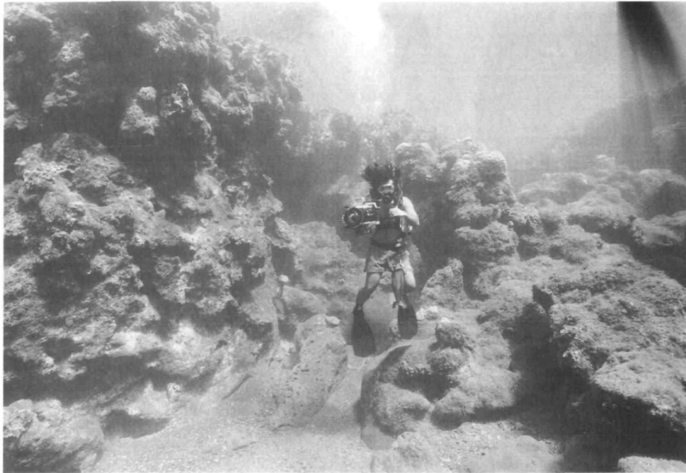
FIG. 2. Coastal reef off Southern Guam which was killed by sedimentation. A fairly dry typhoon removed sediment accumulations from the reef.
