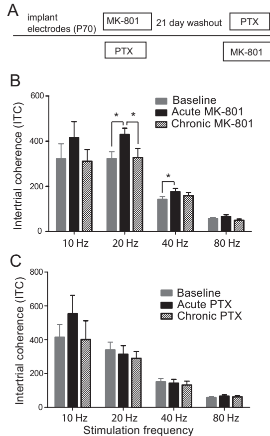
Figure 3. Effect of acute and chronic MK-801 and picrotoxin (PTX) on primary auditory (A1) cortex intertrial coherence (ITC) during auditory steady-state response (ASSR). (A) Timeline showing MK-801 and PTX treatment. All animals received both drugs in a counter-balanced design with a washout period of 21 days between each treatment. (B) Mean intertrial coherence (ITC) values at 10-, 20-, 40-, and 80-Hz stimulation frequencies from 11 rats at baseline, after acute MK-801 (0.1 mg/kg i.p.), and after 21-day (chronic) MK-801 treatment (0.1 mg/kg i.p.). Baseline data are average values of the 3 baseline sessions for each animal, while acute and chronic data are from single sessions. ITC at 20- and 40-Hz stimulation frequencies was elevated after acute, but not chronic, MK-801. There was no significant effect of MK-801 at 10 or 80 Hz. (C) Mean ITC values at 10-, 20-, 40-, and 80-Hz stimulation frequencies from 11 rats at baseline, after acute PTX (0.5 mg/kg i.p.), and after 21-day chronic PTX (0.5 mg/kg i.p.). Baseline data shown are average values of the 3 baseline sessions for each animal, while acute and chronic data are from single sessions. There was no significant effect of PTX at any stimulation frequency tested. All data are plotted as mean \pm SEM in this and subsequent figures. * P < .05 .
