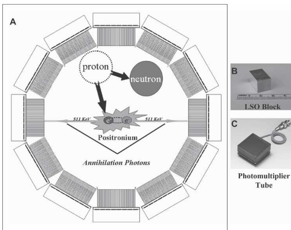
Figure 2 PET scanner detector geometry and positron emission. (A) A PET scanner measures the signal that results from positron ( e^+ ) emission, which occurs when an unstable nucleus decays by emitting a positron, converting a proton to a neutron. The emitted positron combines with an electron to form the ultrashort-lived positronium. Positronium annihilation (mass is converted into energy) creates two 511-keV annihilation photons that are emitted approximately 180^\circ opposed to one another. PET scanners consist of radiation detectors arranged in a geometry that approximates a cylindrical shape. The most common detector type is a block detector, which consists of 50 or more individual elements, or crystals, made of scintillation material, and electronics that determine which individual crystal was struck by a photon. The individual detector elements in the PET scanner operate in coincidence to detect the 511-keV annihilation photons. The detection of coincidence events identifies a line of response in which the decay occurred. This figure also shows a sample lutetium oxyorthosilicate (LSO) inorganic scintillator block of crystals (B) and (C) a photomultiplier tube coupled to the detector block to collect scintillation light for crystal identification.
