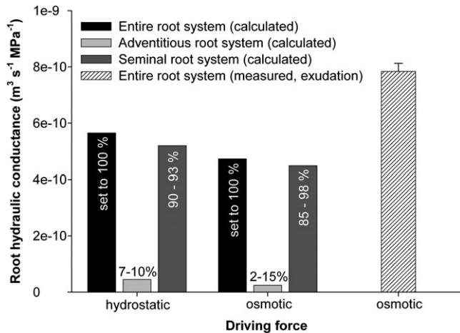
Fig. 4. Contribution of seminal and adventitious roots to water uptake in 14- to 17-d-old barley plants in dependence on the driving force (osmotic, hydrostatic). Hydraulic conductance was determined through osmotic and hydrostatic experiments for individual seminal and adventitious roots (see Table 3). The average values of these experiments were then used to calculate the hydraulic conductance of a typical seminal and a typical adventitious root system of a barley plant, containing 6–7 (average 6.5) seminal and 2–4 (average 3) adventitious roots, respectively. The sum of the two gave the conductance of the entire root system of a plant. Percentage figures give the contribution of the conductance of the seminal and adventitious root system to the conductance of the entire root system of a barley plant. The range of conductance values, as calculated from the range of means given in Table 3 was as follows (unit: \text{m}^3 \text{s}^{-1} \text{MPa}^{-1} \times 10^{-10} ): hydrostatic force, seminal roots, 4.2–6.1; adventitious roots, 0.45 (results from only one analytical method used); entire root system of plant, 4.7–6.6; osmotic force, seminal roots, 1.8–7.7; adventitious roots, 0.18–0.30; entire root system of plant, 2.0–8.0. Also shown is an experimentally (exudation) determined osmotic hydraulic conductance for an entire barley root system; average and SD (error bars) of four independent root analyses.
