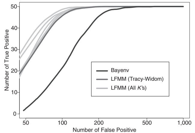
Fig. 4. Spatial coalescent simulations with loci under selection. Number of true positive associations for BAYENV and for LFMM for K = 5, 7 (STRUCTURE and Tracy–Widom values) and for K = 1, 3, 10 , and 20 for spatial coalescent simulations including 1,050 loci with 50 SNPs under selection.
