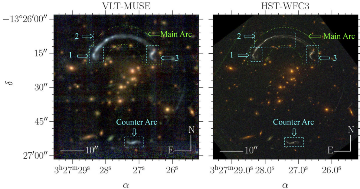
Figure 1. Left: Coloured image of RCS0327 from the MUSE data cube. Three narrowband images of 100 \text{ \AA} width are combined to create an RGB image. The blue, green, and red narrow bands are centred at 4850, 6050, and 8050 \text{ \AA} , respectively. Right: Coloured image of the same field using Hubble Space Telescope ( HST ) Wide Field Camera 3 (WFC3) F390W, F606W, and F814W filters. The main arc is marked with a dotted green polygon. The dashed cyan rectangles mark the multiple images due to lensing of the target galaxy.
