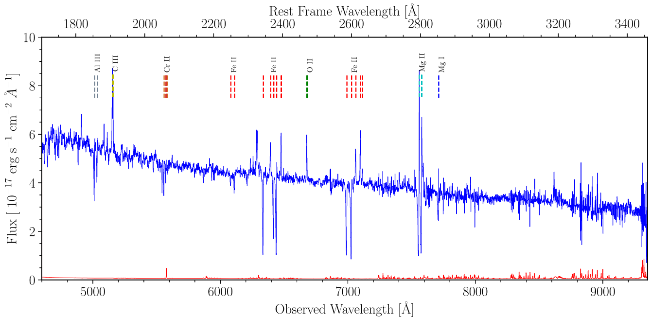
Figure 4. White light-weighted spectrum of the main arc from the MUSE data cube. The flux is shown as a solid blue line and the error is shown as a solid red line. The dashed coloured lines represent the detected emission or absorption transitions in the spectrum, and each distinct colour represents one ionic species. This integrated spectrum has a high SNR of 86, and even the weaker Fe II 2249 line is detected. In our analysis, we exclusively use the [O II], Fe II, and Mg II lines from MUSE observation. We mark the rest of the lines in the spectrum for completeness. All the transitions shown in this Figure are summarized in Table 1.
