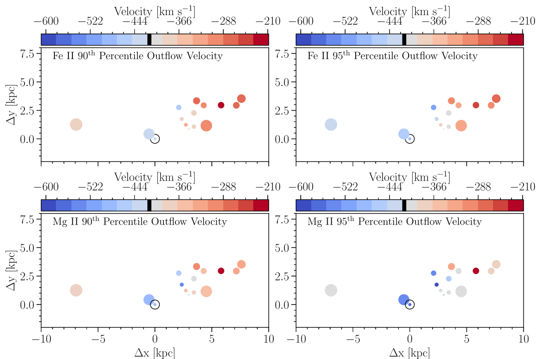
Figure 9. Extreme outflow velocities in the source-plane. The x- and y-axes represent the physical distance in the source-plane for all panels. Top row: The 90 th ( Left ), and the 95 th ( Right ) percentile velocities for the Fe II outflow component. Bottom row: The 90 th ( Left ), and the 95 th ( Right ) percentile velocities for the Mg II outflow component. The colours of the data points represent the value of the velocity (see colour bar above plots). The sizes of the data points represent the areas of the selected regions in the source-plane. The data points with black open circles around them represent the global values from the spectrum of the counter arc. The black vertical band in each colour-bar represents the value for the escape velocity ( V_{\text{esc}} = -418 \text{ km s}^{-1} ) at 5 kpc.
