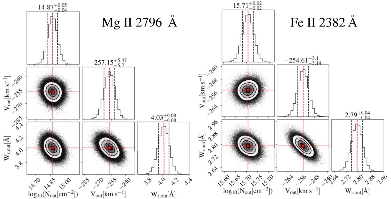
Figure 7. Posterior probability distribution functions (PPDFs) showing the outflow properties for both Mg II (Left) and Fe II (Right) from the counter arc spectrum. PPDFs of outflow velocity ( V_{\text{out}} ), outflow column density ( \log_{10}(N_{\text{out}}) ) and outflow equivalent widths ( W_{r,\text{out}} ) are presented. These measurements represent the average global outflow properties in the galaxy. The outflow velocity measurement from Mg II and Fe II are consistent with each other within the error bars. The error-bars on \log_{10}(N_{\text{out}}) represent the uncertainty from model fitting. The Mg II column densities are poorly constrained due to saturation of the lines (see Fig. 6).
