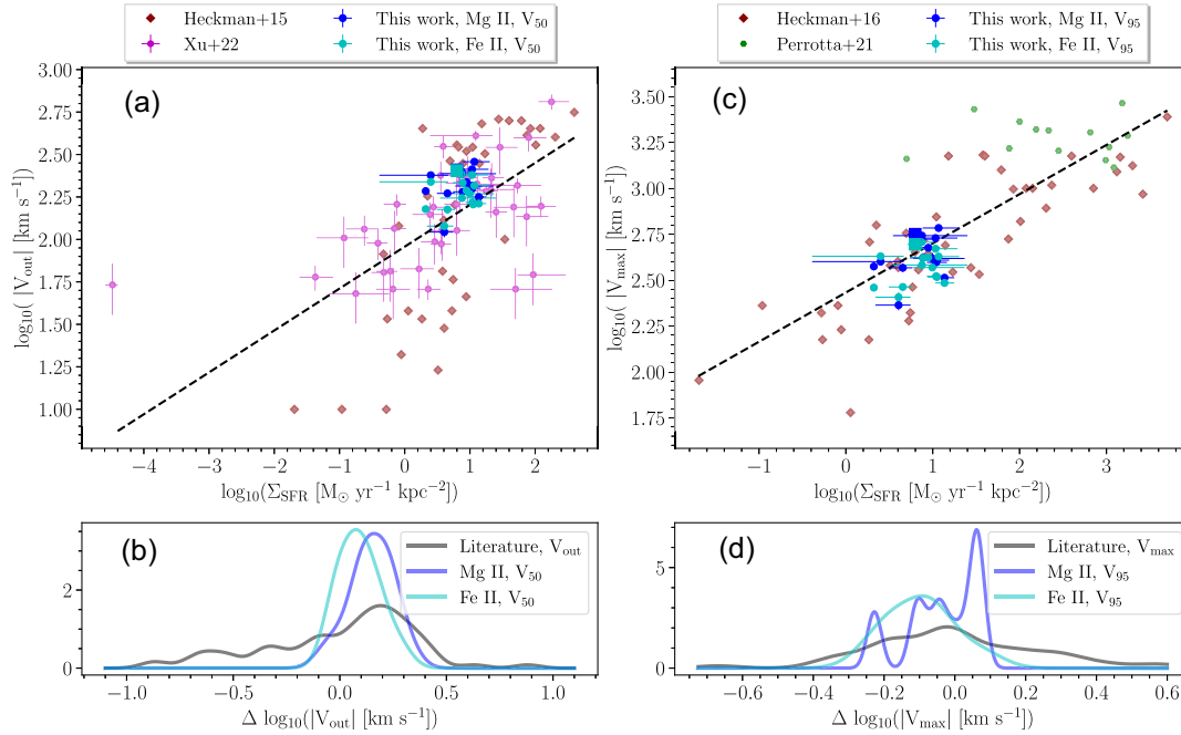
Figure 14. Panel (a): 50th percentile outflow velocity versus SFR per unit area ( \Sigma_{\text{SFR}} ). The blue and cyan circles represent the outflow velocity for Mg II and Fe II in RCS0327, respectively. The cyan and blue squares are the average measurements of the counter arc for Fe II and Mg II, respectively. The literature data points in this panel are from Heckman et al. (2015) (brown diamonds), and Xu et al. (2022) (magenta circles). The black-dashed line is the best fit line for the literature data points. Panel (b): KDE of the residual outflow velocity with respect to the literature best fit line ( \Delta \log_{10}(|V_{50}|) = \log_{10}(|V_{50}|) - \log_{10}(|V_{50, \text{best-fit}}|) ) for Mg II (blue curve), Fe II (cyan curve) from RCS0327, and the literature measurements (black curve). The blue and cyan circles are for the Mg II and Fe II for RCS0327, respectively. The literature measurements and medians of their residual distributions are offset from the literature values by -0.1 dex and -0.2 dex for Mg II and Fe II, respectively. From RCS0327, the scatter has a width of \approx 0.9 dex, which is slightly smaller than the width of the scatter of the literature data points that has a width of \approx 1.5 dex. Panel (c): Maximum outflow velocity versus \Sigma_{\text{SFR}} . The literature measurements are from Heckman & Borthakur (2016) (brown diamonds), and Perrotta et al. (2021) (green hexagons). The maximum velocities here have the same definition as in Fig. 13. Panel (d): KDE of the residual maximum outflow velocity with respect to the literature best fit line ( \Delta \log_{10}(|V_{\text{max}}|) = \log_{10}(|V_{\text{max}}|) - \log_{10}(|V_{\text{max, best-fit}}|) ) with the same colour scheme panel (b).
