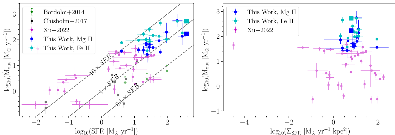
Figure 11. Left: Mass outflow rate \dot{M}_{out} versus the SFR for Mg II (blue circles), and Fe II (cyan circles) for RCS0327 in log scale. The blue and cyan squares in both panels represent the measurements for the counter arc for Mg II and Fe II, respectively. The magenta diamonds and grey squares are from Xu et al. (2022) and Chisholm et al. (2017), respectively. The green diamonds are lower limits for \dot{M}_{out} from Bordoloi et al. (2014b). The black diagonal lines in the panel represent the mass loading factor values ( \eta = \dot{M}_{out}/SFR = 0.1, 1, 10 ). Right: Mass outflow rates versus SFR per unit area \Sigma_{SFR} , in log scale. The colours of the data points are the same as the left panel. In both panels, we see the consistency with respect to the trends of the data reported in Xu et al. (2022). Since the \dot{M}_{out} measurements from RCS0327 are lower limits, this implies that RCS0327 is likely located along the mass loading factor of \eta \sim 10 as seen from the individual regions.
